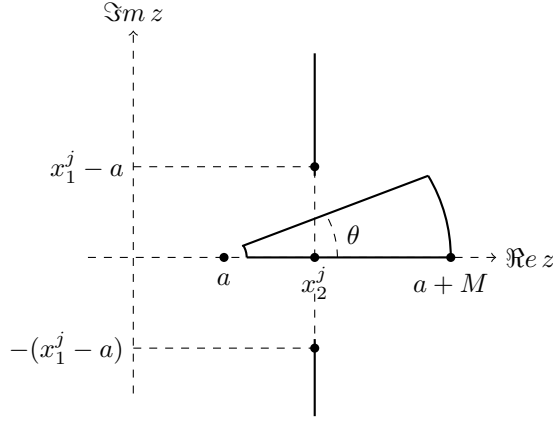
FIG. 5. The contour \partial T_\theta^{\delta, M} and the branch points z_\pm = x_2^j \pm i(x_1^j - a) of h(x_1^j - a, x_2^j - z) .
