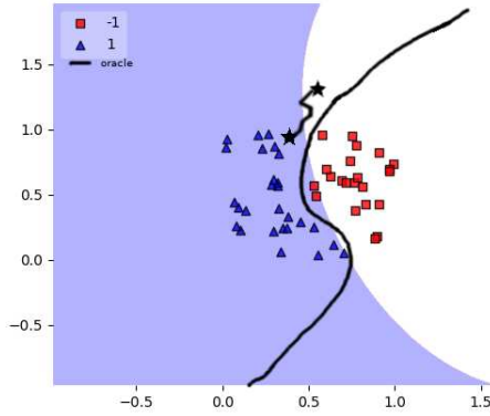
Fig. 3: Adversarial configurations (stars) are at the limit of the separating function learned by the ML classifier
