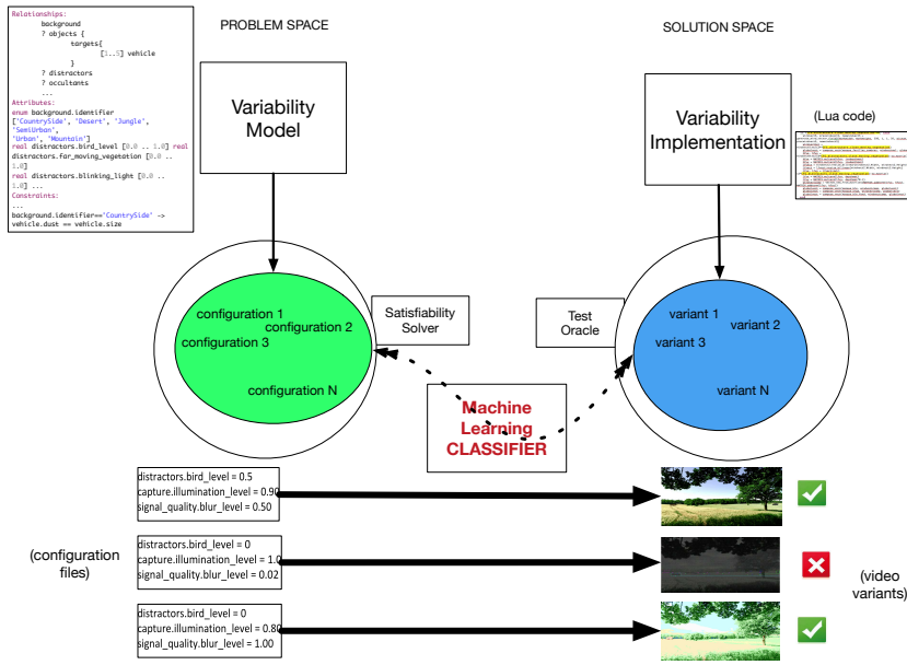
Fig. 2: Software product line and ML classifier
