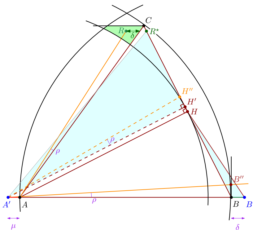
Figure 6: Lemma 9.
