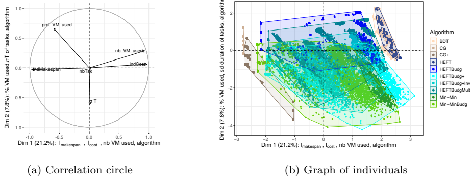
Figure 3: Correlation circle and graph of individuals for schedules obtained for MONTAGE workflows of 60 tasks
