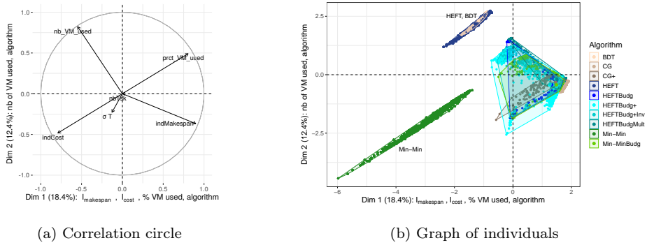
Figure 4: Correlation circle and graph of individuals for schedules obtained for LIGO workflows of 60 tasks
