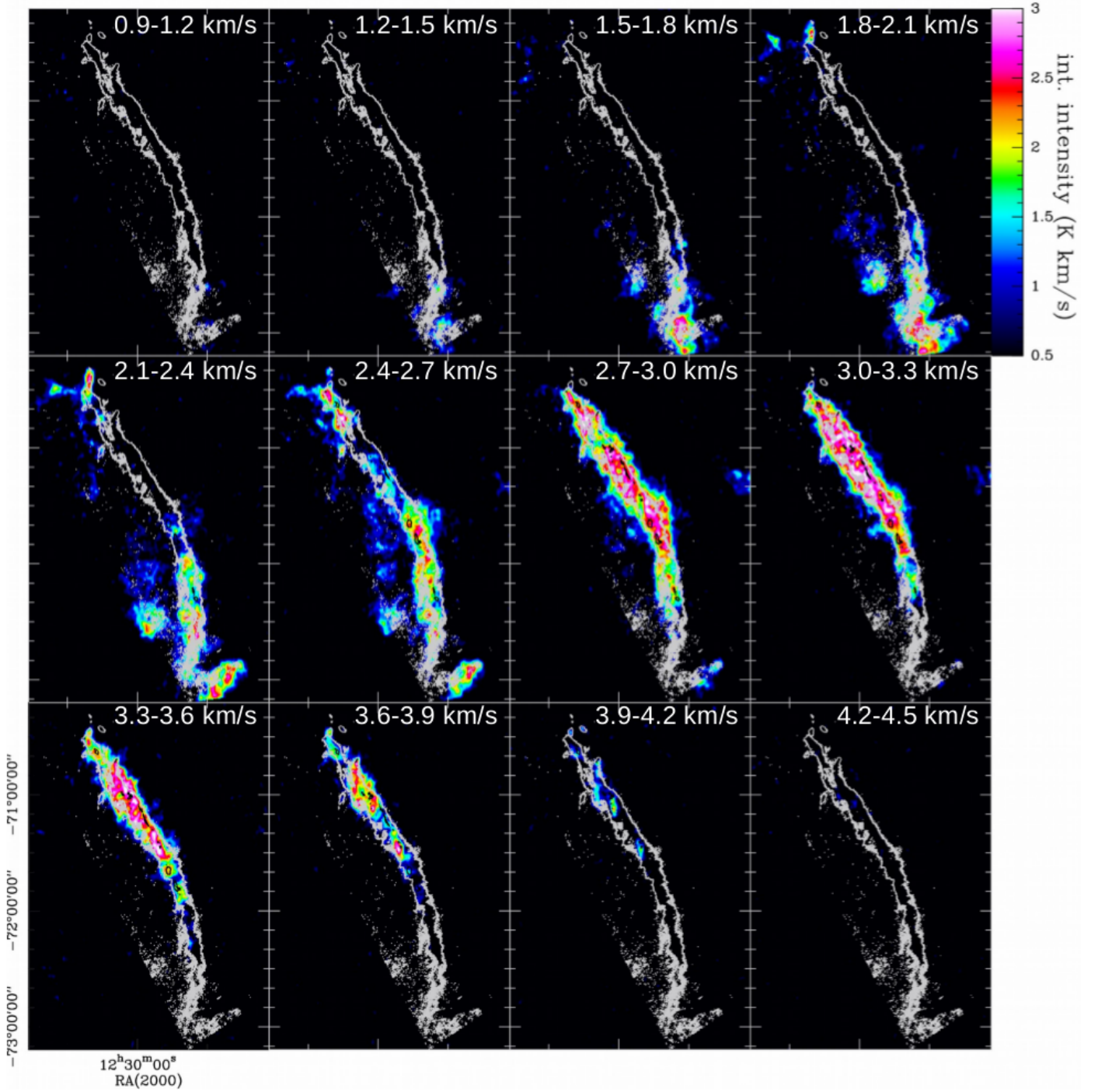
Fig. 12. Integrated intensity of NANTEN2 data over velocity intervals of 0.3 \text{ km s}^{-1} . The black contours at N_{\text{H}_2} = 5 \cdot 10^{21} \text{ cm}^{-2} from the Herschel data indicate the center of the filament crest. These black contours are best visible at velocities between 2.7 and 3.6 \text{ km s}^{-1} when there is ^{12}\text{CO}(1-0) emission towards the crest. The grey contour, at N_{\text{H}_2} = 2 \cdot 10^{21} \text{ cm}^{-2} , indicates the area that encloses the strands. It can be observed that there is some extended emission east of the Musca filament and that the filament crest is not at the middle of the area containing the strands.
