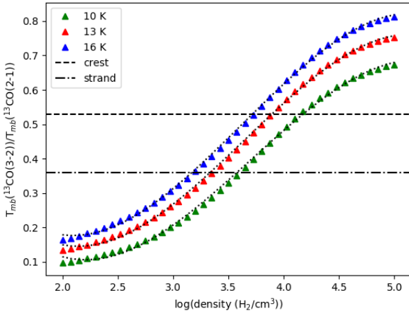
Fig. 15. Evolution of the ^{13}\text{CO}(3-2)/^{13}\text{CO}(2-1) brightness temperature ratio as a function of density for realistic temperatures of the Musca filament. The dotted curves are the functions fitted through the RADEX results to invert the observed ratio in Musca to a density. The horizontal lines indicate the average observed ratios for the strand and the crest in the northern map.
