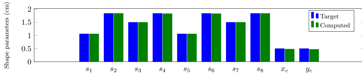
Figure 7: Characteristic shape parameter values of the octagonal-shaped scatterer experiment. Target vs. Computed Values at convergence. f = 55.7\text{kHz} and noise free measurements.
