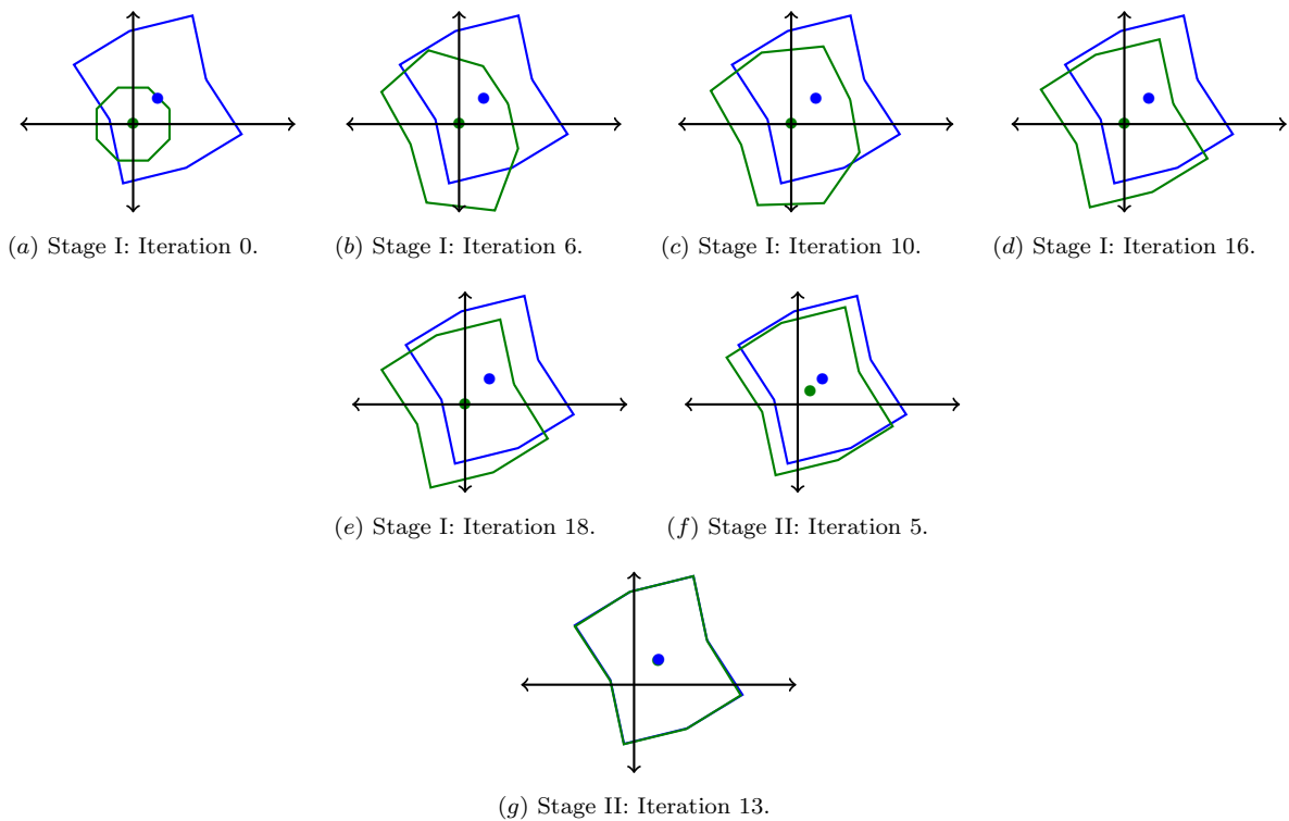
Figure 6: Shape and location of the octagonal-shaped scatterer experiment. Target vs. Computed Values at the occurred stagnations. f = 55.7\text{kHz} and noise free measurements.
