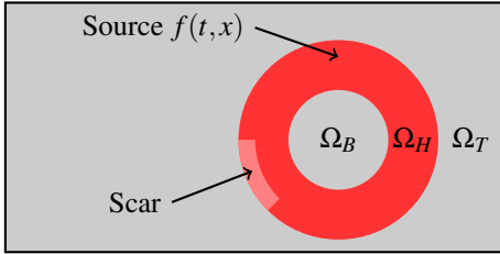
Figure 1. Sketch of the model with a scar.
