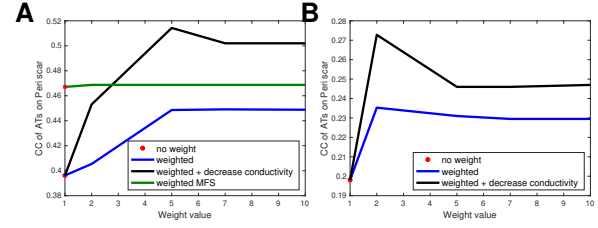
Figure 6. CC only on the neighborhood of the scar, four pacing sites, left ventricular scar. CC for 1 \leq w \leq 10 (MFS in green, VM with \rho = 1 in blue, VM with \rho = 0.1 in black). A: Epicardium. B: Endocardium
