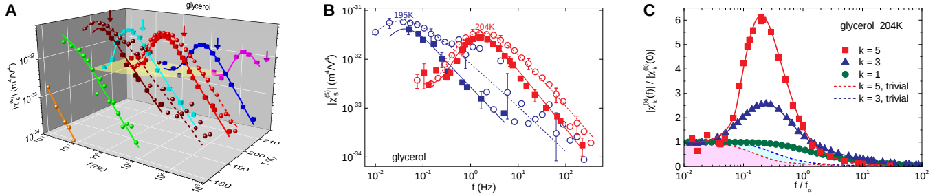
FIG. 12. Modulus of the fifth-order susceptibility in super-cooled glycerol as a function of frequency (from [161]). (A) The susceptibilities \chi_5^{(5)} reported are obtained directly by monitoring the response of the sample at 5\omega , when applying an electric field E at angular frequency \omega . Two independent setups were used. Lines are guides for the eyes. (B) Projection onto the susceptibility-frequency plane of the data of panel A at 204K and at 195K. (C) Comparison of the fifth-order, cubic, and linear susceptibilities. Symbols, with line to guide the eyes. The higher the order k , the stronger the hump of |\chi_k^{(k)}| .
