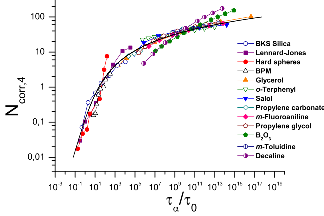
FIG. 11. Universal dynamic scaling relation between number of dynamically correlated particles, N_{\text{corr},4} , and relaxation timescale, \tau_\alpha , for a number of glass-formers [150], determined using Eq. (12).
