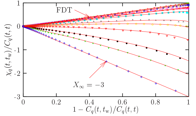
FIG. 24. Parametric response-correlation plots for the Fourier components of the mobility field in the d = 3 Fredrickson-Andersen model. Symbols are from simulations, lines from analytic calculations, and wavevectors decrease from top to bottom. The FDT is close to being satisfied at large q corresponding to local equilibrium. At larger distance deviations from the FDT are seen, with an asymptotic FDR which becomes negative. Finally, for energy fluctuations at q = 0 (bottom curve), the plot becomes a pure straight line of (negative!) slope -3 , as a result of thermally activated dynamics.
