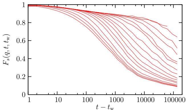
FIG. 21. Aging dynamics in a Lennard-Jones glass-forming liquid at low temperature. The system is quenched at time t_w = 0 at low T , where the temperature is kept constant. Two-time self-intermediate scattering functions are then measured for 20 logarithmically spaced waiting times t_w from t_w = 1 to t_w = 10^5 (from left to right). The relaxation becomes slower when t_w increases: the system ages.
