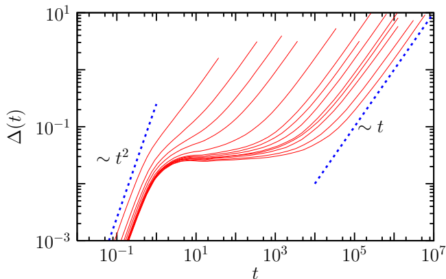
FIG. 4. Mean-squared displacements of individual particles in a simple model of a glass-forming liquid composed of Lennard-Jones particles observed on a wide time window. When temperature decreases (from left to right), the particle displacements become increasingly slow with several distinct time regimes corresponding to (in this order) ballistic, localized, and diffusive regimes.
