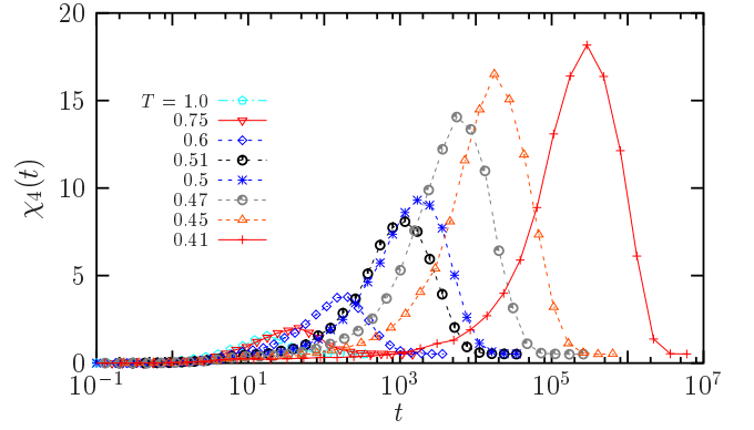
FIG. 10. Time dependence of \chi_4(t) , quantifying the spontaneous fluctuations of the intermediate scattering function in a Lennard-Jones supercooled liquid. For each temperature, \chi_4(t) has a maximum, which shifts to larger times and has a larger value when T is decreased, revealing the increasing lengthscale of dynamic heterogeneity in supercooled liquids approaching the glass transition.
