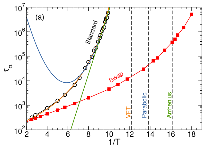
FIG. 18. From [338]. Relaxation times for standard (open symbols) and swap (closed symbols) Monte Carlo dynamics. The standard dynamics is fitted with the VFT, parabolic, and Arrhenius laws, which are then used to estimate the location of the experimental glass temperature T_g (vertical dashed lines). The swap dynamics efficiently equilibrates the system at temperatures below T_g .
