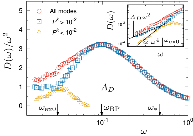
FIG. 17. Adapted from [324]. Vibrational density of states of jammed harmonic soft spheres scaled by the Debye law \omega^{d-1} in d = 3 . Modes with index k are classified as extended (blue) or localized (yellow) by their participation ratio P^k . Below the boson peak frequency \omega_{BP} , the density of states is the superposition of anomalous extended modes eventually obeying Debye scaling, and a population of quasi-localised modes scaling as \omega^4 , as confirmed in the inset.
