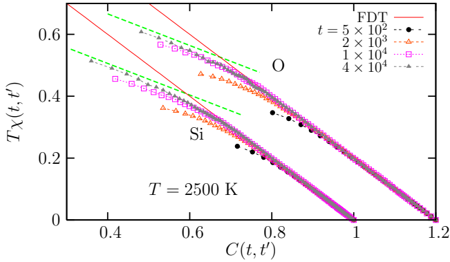
FIG. 23. Parametric correlation-response plots measured in the aging regime of a numerical model for a silica glass, \text{SiO}_2 [423]. The plots for both species smoothly converges towards a two-straight line plot of slope 1 at short times (large C values), and of slope X^\infty \approx 0.51 at large times (small values of C ), yielding an effective temperature of about T_{\text{eff}} = T/X^\infty \approx 4900 K. Note that the glass transition temperature of \text{SiO}_2 is 1446K.
