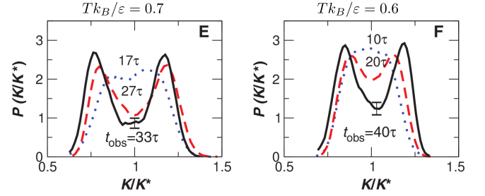
FIG. 20. From [263]. Coexistence of the active (large K ) and inactive (small K ) phases, as evidenced from s -ensemble biased simulations. As temperature is reduced, the distribution becomes increasingly bimodal, as expected when approaching a first order phase transition.
