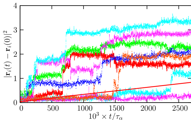
FIG. 7. Time resolved squared displacements of individual particles in a simple model of a glass-forming liquid composed of Lennard-Jones particles. The average is shown as a smooth full line. Trajectories are composed of long periods of time during which particles vibrate around well-defined positions, separated by rapid jumps that are widely distributed in time, underlying the importance of dynamic fluctuations.
