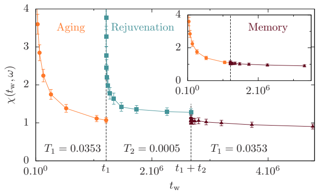
FIG. 22. Memory and rejuvenation effects obtained in the numerical simulation of a three-dimensional glass-former [303]. There is a first aging step, 0 < t_w < t_1 , during which the system slowly tries to reach thermal equilibrium at temperature T_1 . The system ‘rejuvenates’ in the second step at T_2 , t_1 < t < t_1 + t_2 , and it restart aging (rejuvenation). Finally in the third step, temperature is back to T_1 , and memory of the first step is kept intact, as shown in the inset where relaxation during the second step of the experiment is taken away.
