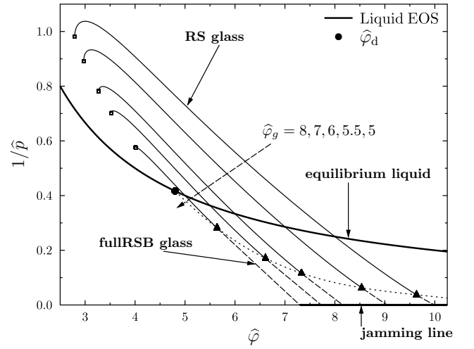
FIG. 16. Phase diagram of hard spheres in the inverse reduced pressure – reduced packing fraction (1/\hat{p}, \hat{\varphi}) plane. The glass transition is marked by a full circle. The glass equations of state are reported as full lines in the region where the replica symmetric solution is stable. The Gardner transition is marked by triangles, beyond which the fullRSB solution is stable (dashed lines). The glass equations of state end at the jamming transition. Upon decompression, glasses are stable until a spinodal instability arises (open squares).
