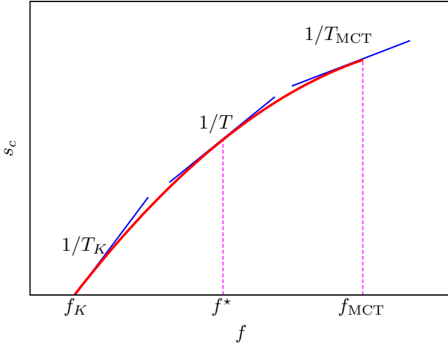
FIG. 14. Typical shape of the configurational entropy, s_c , as a function of free energy density, f in the range T_k < T < T_{MCT} for random first order landscapes. A graphical solution of Eq. (22) is obtained by finding the value of f at which the slope of the curve is 1/T . Note that s_c is also a function of temperature, so this curve changes with T .
