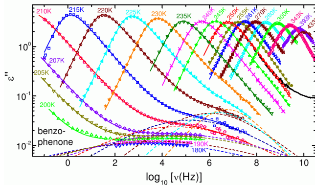
FIG. 3. Temperature evolution of the dielectric susceptibility of the glass-former benzophenone measured over more than 10 decades of relaxation times [20]. Dynamics slows down dramatically as temperature is decreased and relaxation spectra become very broad at low temperature.
