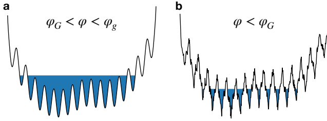
FIG. 15. (a) Sketch of the free energy structure deep in the hard sphere glass phase, where each basin breaks down in sub-basins corresponding to secondary relaxations. At the Gardner transition in (b), the sub-basins become fractal and ergodicity is broken.
