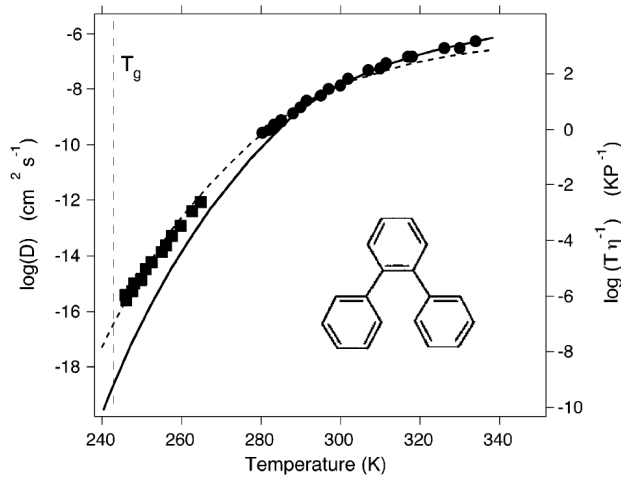
FIG. 8. Decoupling between viscosity (full line) and self-diffusion coefficient (symbols) in supercooled orthoterphenyl [133]. The dashed line shows a fit with a ‘fractional’ Stokes-Einstein relation, D_s \sim (T/\eta)^\zeta with \zeta \sim 0.82 .
