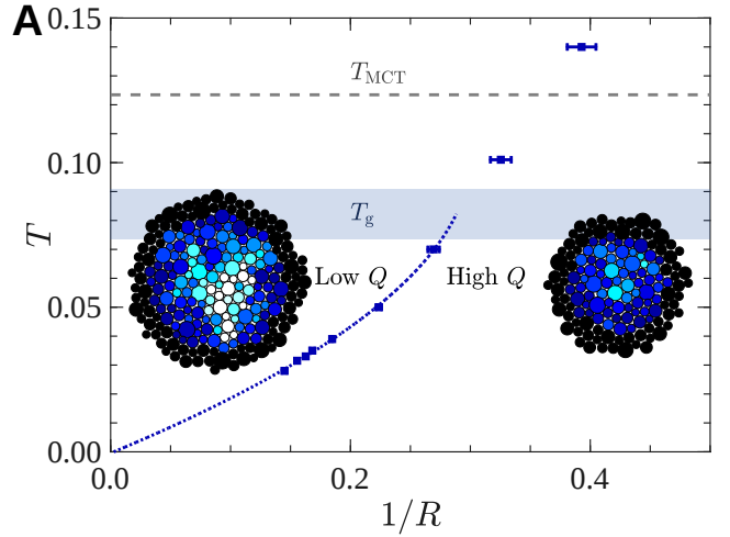
FIG. 19. From [349]. Evolution of the inverse point to set length, denoted here as 1/R with the temperature T . A clear growth of the point to set length up to \xi_{PTS} \approx 6.5 is observed. Cavities smaller (larger) than \xi_{PTS} have a large (small) overlap with the reference configuration, as illustrated in the snapshots, where the particle shade encodes the overlap value.
