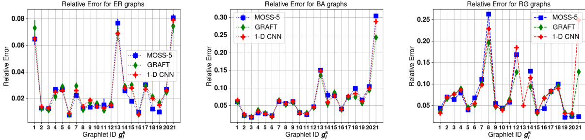
Figure 9: Relative Errors of 1-D CNN and Competing Methods for 5-node graphlets
