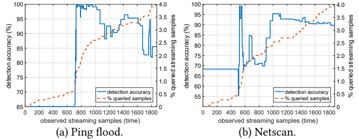
Figure 3: RAL temporal convergence.
