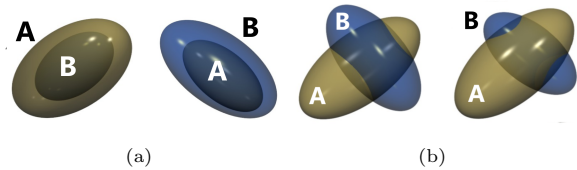
Fig. 4. Each pair of ellipsoids in (a) and (b) are not equivalent.
