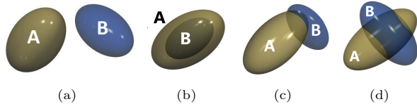
Fig. 2. Four arrangements of two ellipsoids
