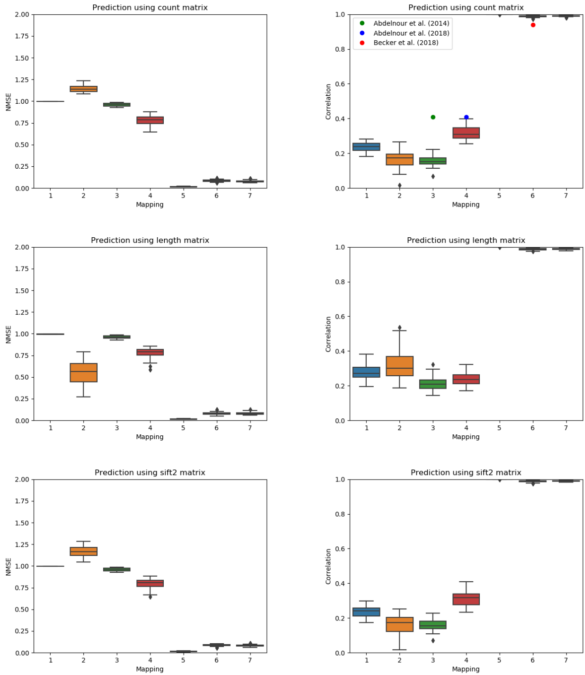
Figure 3: Normalized mean squared error (lower is better) and correlation (higher is better) between the predicted and true functional matrices for some of the mapping of Table 1 for single-subject testing. The mappings using a mean are omitted. The mean correlation reported by previous publications are illustrated using circles in the column corresponding to their model.
