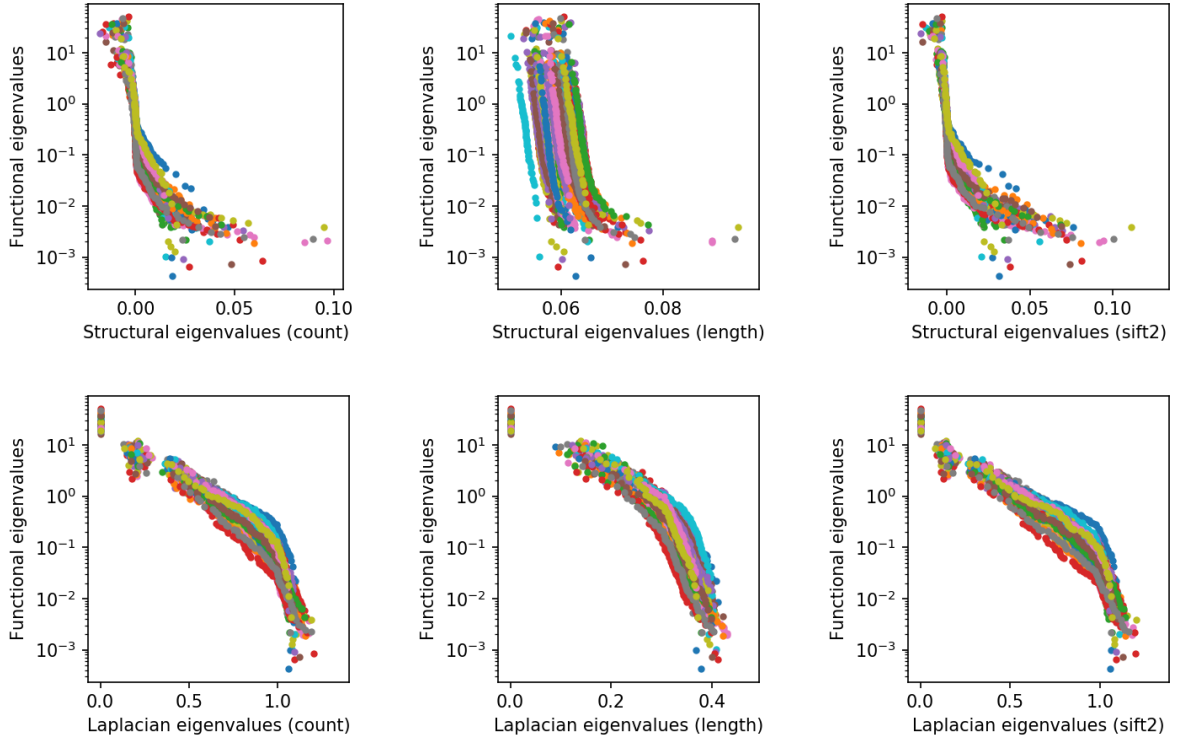
Figure 2: Functional eigenvalues as a function of the structural and Laplacian eigenvalues. Each dot corresponds to one eigenvalue pair with the colors corresponding to subjects. The top row relates the eigenvalues of the functional connectivity matrix directly to those of the structural connectivity matrix whereas the bottom row relates them to the eigenvalues of the Laplacian of the structural connectivity matrix. Note the use of a logarithmic scale for the ordinates.
