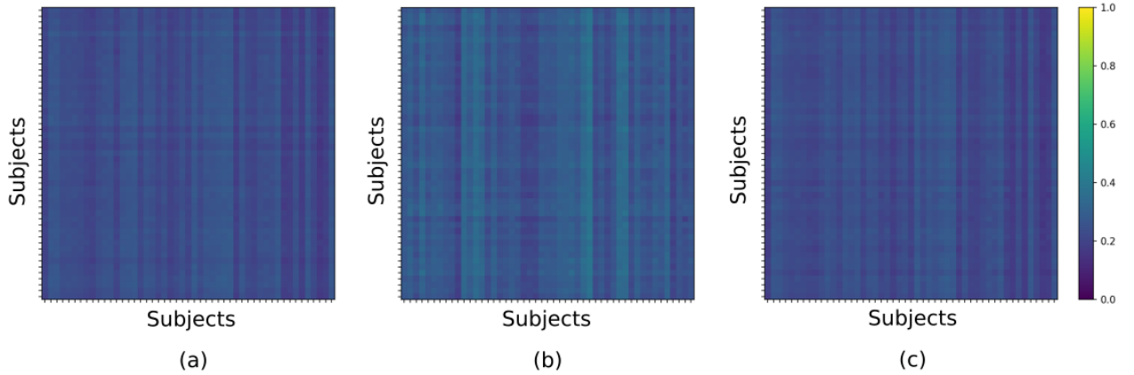
Figure 1: Illustration of the inter-subject correlation between the functional connectivity matrix and the count (a), length (b), and SIFT2 (c) matrices.
