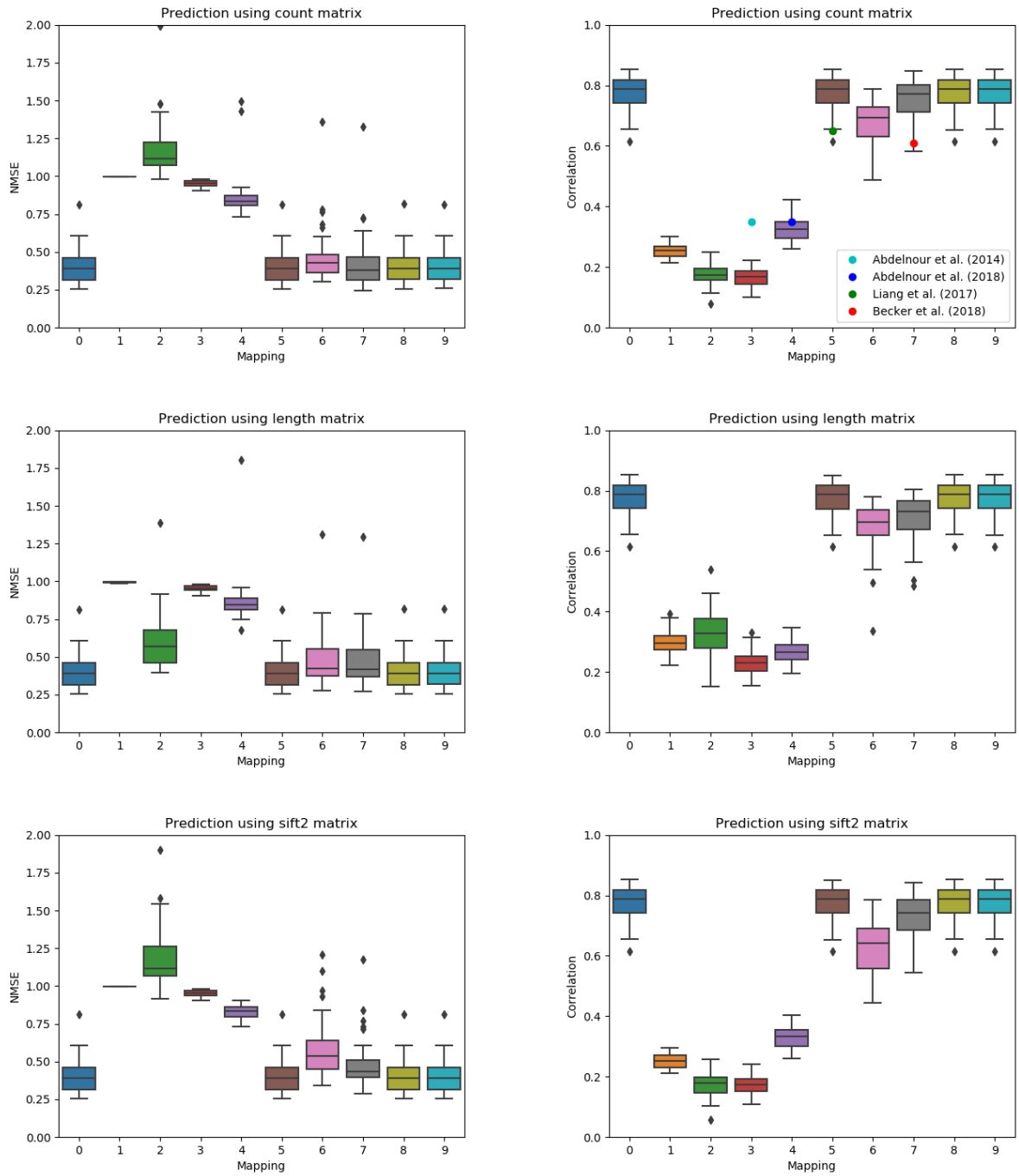
Figure 4: Normalized mean squared error (lower is better) and correlation (higher is better) between the predicted and true functional matrices for each mapping of Table 1 for multi-subject testing. The mean correlation reported by previous publications are illustrated using circles in the column corresponding to their model.
