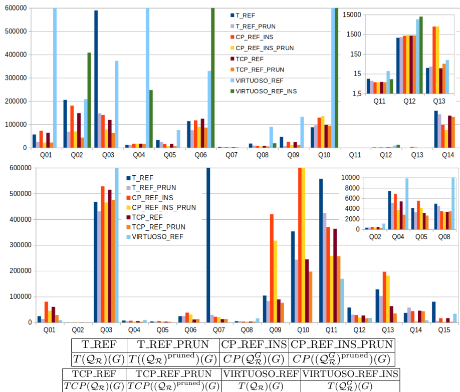
Fig. 3. LUBM (top) and DBLP (bottom) query answering times (ms) through reformulation.
