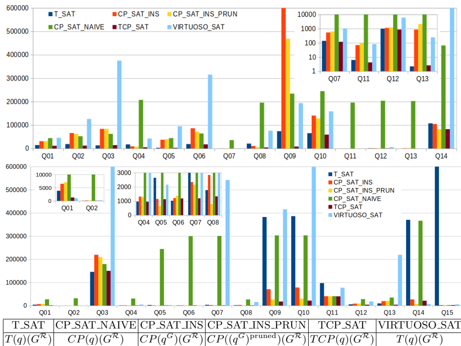
Fig. 2. Query answering times (milliseconds) on LUBM (top) and DBLP (bottom), through saturation.
