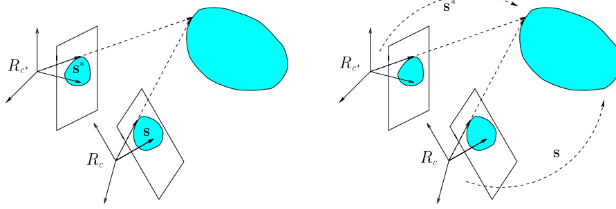
Fig. 2 If the goal is to move the camera from frame R_c to the desired frame R_{c^*} , two main approaches are possible: IBVS on the left, where the features \mathbf{s} and \mathbf{s}^* are expressed in the image, and PBVS on the right, where the features \mathbf{s} and \mathbf{s}^* are related to the pose between the camera and the observed object.
