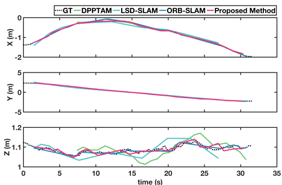
Fig. 6: Comparison of trajectories generated from different methods: Our proposed method shows a more stable and similar trajectory results w.r.t LSD-SLAM and DPPTAM, reaches the save level of state-of-the-art sparse SLAM method ORB-SLAM, thanks to the global planar representation and non-linear BA.
