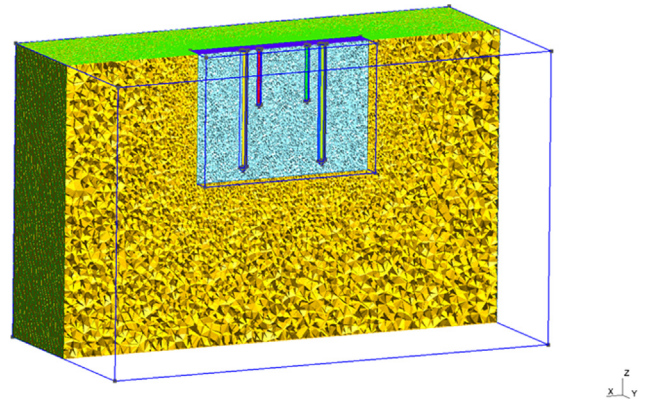
Fig. 3. 3D mesh of the 4-electrode finite element model.
