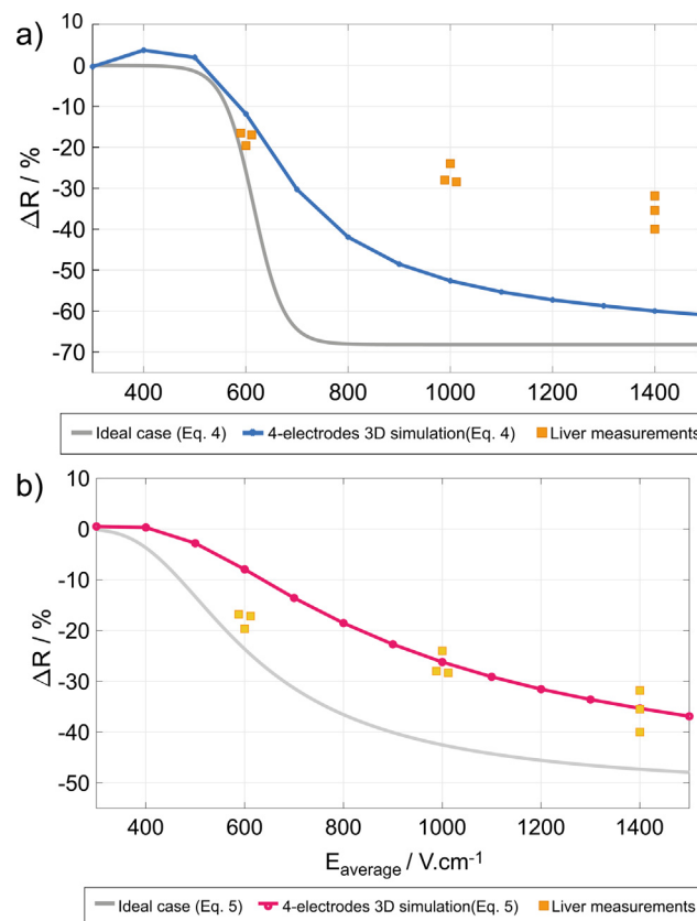
Fig. 6. Variation of the simulated equivalent resistance R_{\text{eq}} for the 4-electrodes system. The liver measurements correspond to the measured experimental resistance R_{\text{pulse}} at the end of the pulse (data from Table 1, three different animal per field condition). Additionally, the ideal case corresponding to the resistance between two parallel plates of infinite extent is shown for comparison. (a) The non-linear model for the tissue conductivity given by Eq. (4) is used in the simulation ( a = 650 V/cm and b = 30 V/cm). (b) The electroporation model for the conductivity given by Eq. (5) is used in simulations ( a' = 800 V/cm). In both models, \sigma_{\text{ext}} = 0.07 S/m and \sigma_{\text{int}} = 0.15 S/m.
