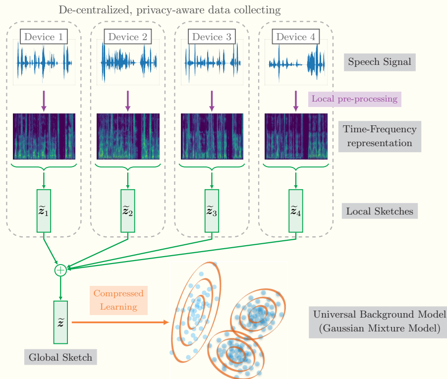
Fig. 6: Speaker verification with sketching. Unlabeled training speech data is collected in a decentralized manner, pre-processed and sketched locally. The local sketches are then merged and a Universal Background Model is learned from the global sketch.
