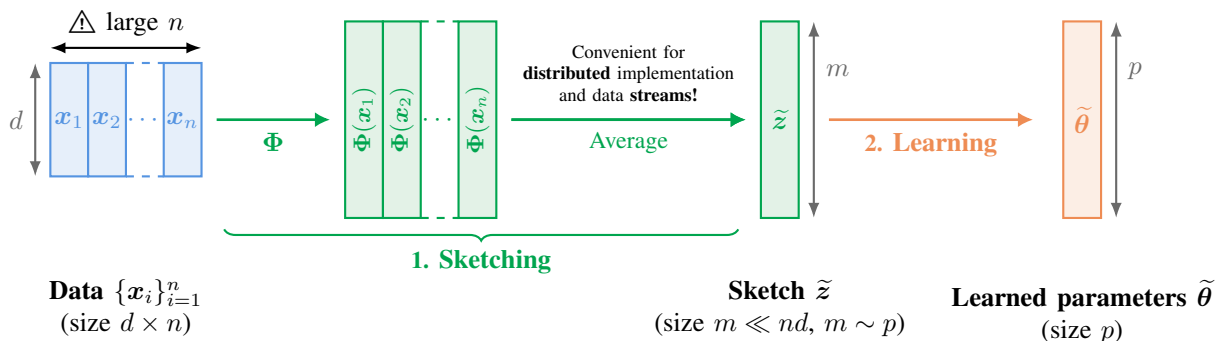
Fig. 1: Overview of sketching and parameter learning.
