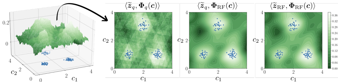
Fig. 13: Criterion \langle \tilde{\mathbf{z}}, \Phi(\mathbf{c}) \rangle versus centroid hypothesis \mathbf{c} = [c_1, c_2]^\top used by greedy parameter estimation algorithms in sketched clustering with k = 3 and a 2D dataset (in blue), with and without quantization of the sketch \tilde{\mathbf{z}} and/or feature map \Phi . The surface plot on the left highlights the irregularity of \mathbf{c} \mapsto \langle \tilde{\mathbf{z}}_q, \Phi_q(\mathbf{c}) \rangle .
