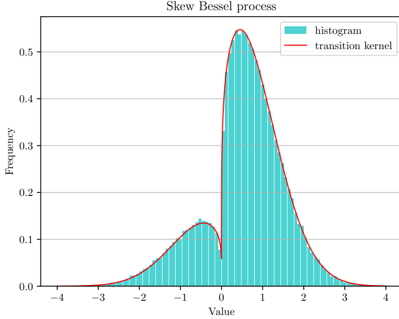
Figure 6: Histogram of simulated values at T = 1 of the Skew Bessel process of parameters (\delta, \beta) = (1.2, 0.8) with initial value x_0 = 0 using Algorithm 1 with a uniform grid of step-size h = 0.01 . The quantities (56) were approximated using 100-step Riemann approximations.
