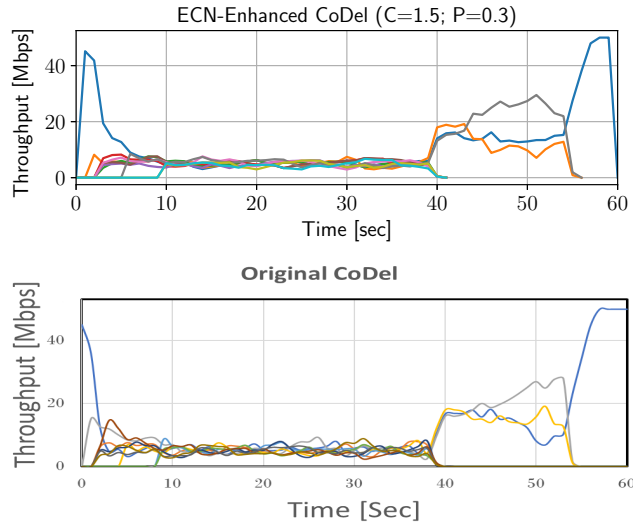
Fig. 11. Throughput with ECN-enhanced/Original CoDel (10-TCP flows)
