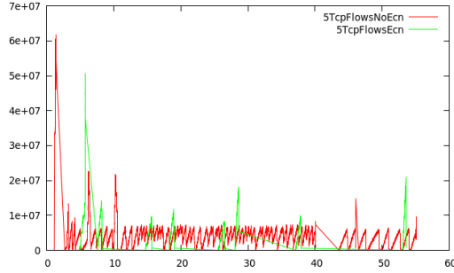
Fig. 10. Sojourn Time (5-TCP flows).
