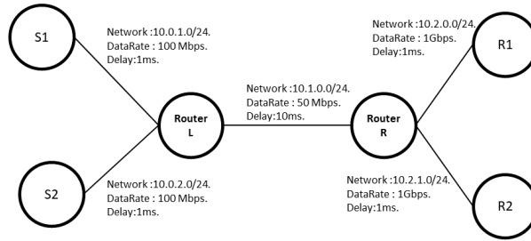
Fig. 2. Network Topology.
