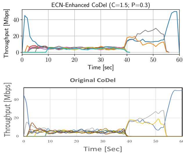
Fig. 11. Throughput with ECN-enhanced/Original CoDel (10-TCP flows)
