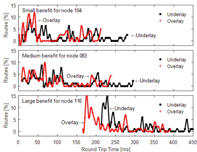
Fig. 3: Variations of RTT Benefit
