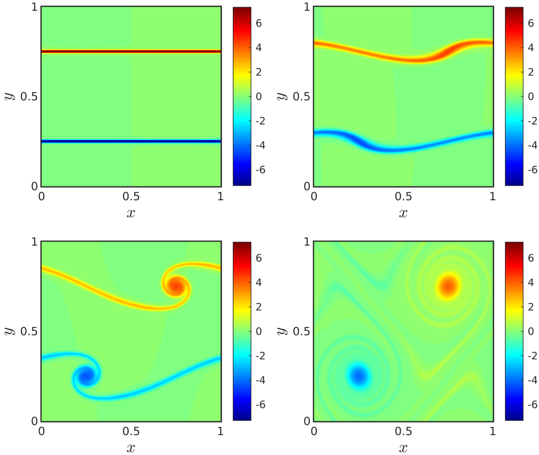
Figure 1. Spatial distribution of \omega_z/\sqrt{\Omega_{ref}} for case r160 at 4 instants t\sqrt{\Omega_{ref}} = \{0, 7, 10, 23\} in the following respective order: top left, top right, bottom left and bottom right.
