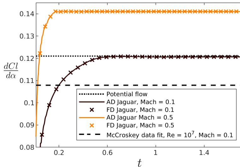
Figure 4. Sensitivity of the lift coefficient Cl to a change in incidence angle \alpha around a NACA 0012 airfoil at zero incidence. Two Mach numbers considered, sensitivities computed with FD and JAGUAR differentiated in tangent-mode AD. Values are compared with the curve fit to experimental data from [22], and with the solution found using FD with the panel code XFOIL (potential flow). Time t is in code units. We verified that the agreement between the JAGUAR output at Ma = 0.1 and Ma = 0.5 is considerably improved if normalized by the low Ma correction factor \sqrt{1 - (Ma)^2} .
