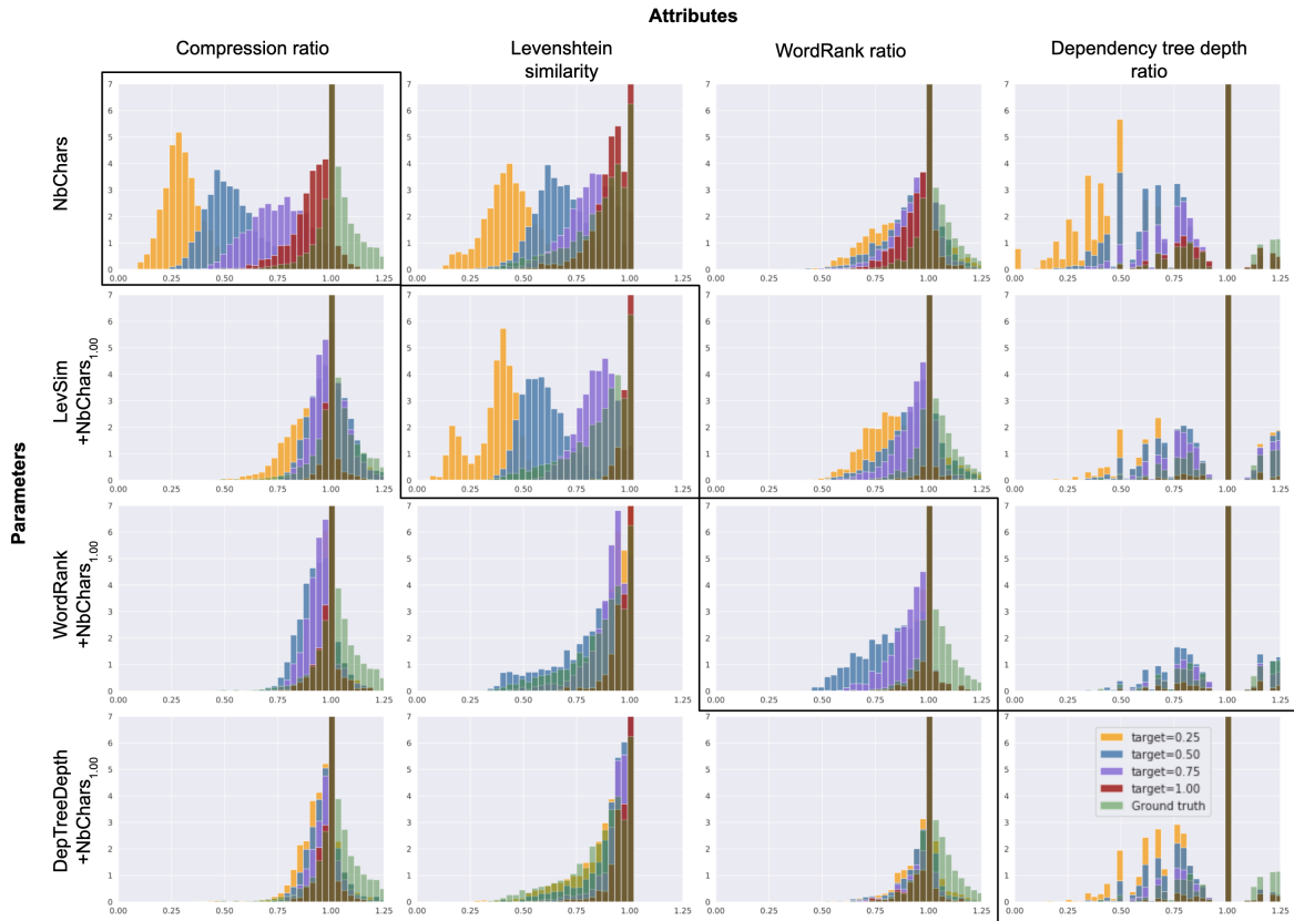
(a) With the NbChars 1.00 constraint.
