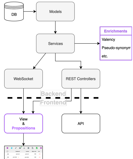
Figure 2: User Interface architecture for OFrLex validation
