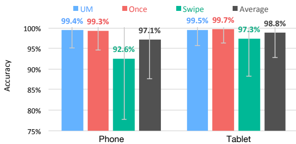
Figure 7: Accuracy performance for individual input method on both phone and tablet for the two-handed conditions. Error bars show 95% confidence intervals. Ordinate axis starts at 75%
