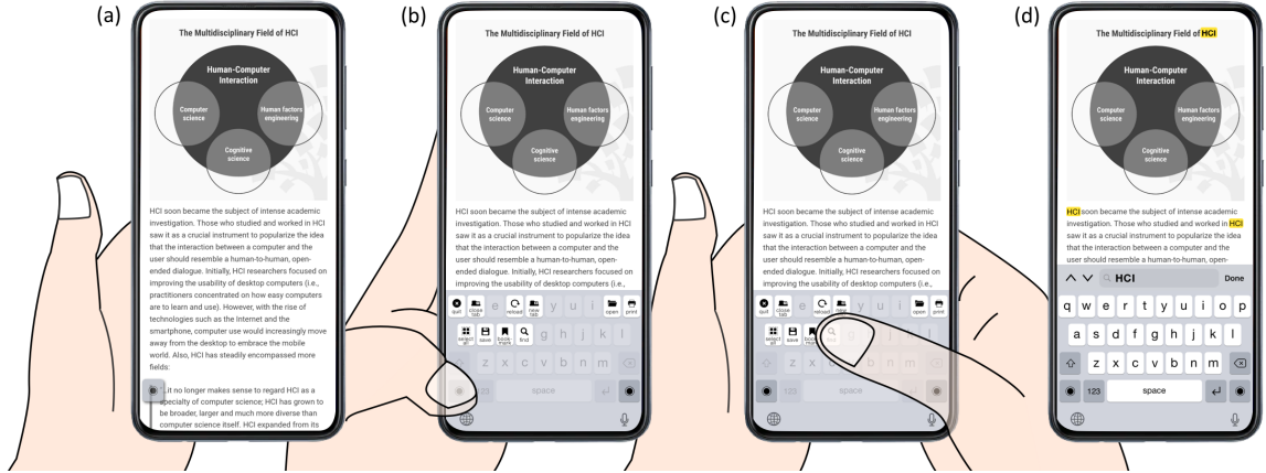
Fig. 1. Web browsing scenario of soft keyboard shortcuts using Once method. (a) a semi-transparent modifier key is available in the browser, (b) when user taps it, all available shortcuts will be presented to facilitate browsing, (c) user then taps on the “F” key (find command) and hence, (d) every occurrence of the “HCI” word (as typed by the user) is highlighted in yellow.
