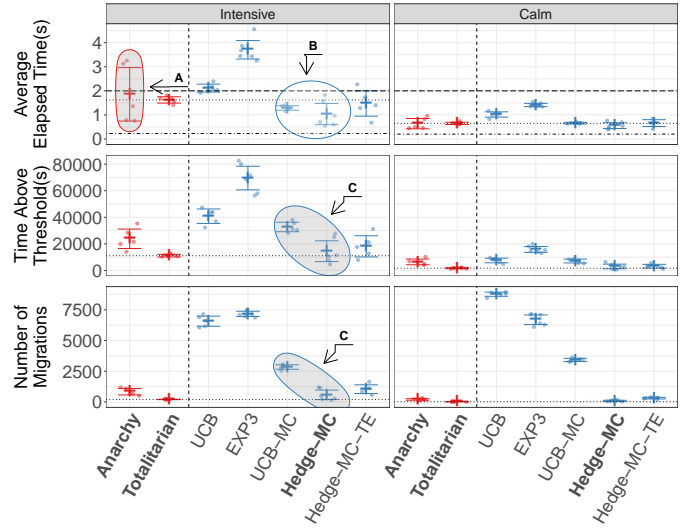
Fig. 16: Performance Evaluation for Learning Strategies in the Affinity Scenario.
