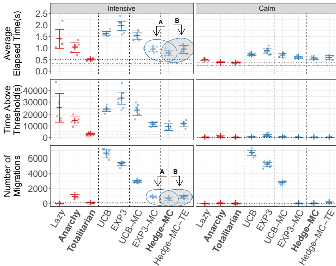
Fig. 12: Performance Evaluation for Hedge-MC and Hedge-MC-TE Strategies. A new metric "Time Above Threshold" is presented.
