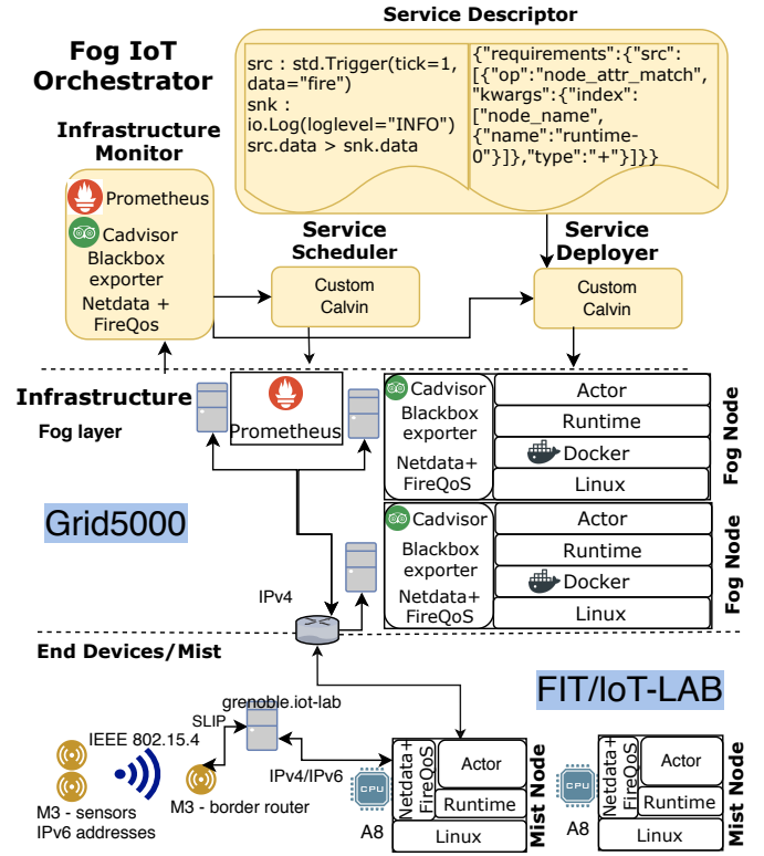
Fig. 4: Fog-IoT Orchestrator Architecture
