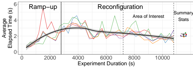
Fig. 3: Performance Evolution for a Reconfiguration Strategy. In Summary Stats, we summarize the average performance during the area of interest, either for each experiment (color dots) or in general (black).
