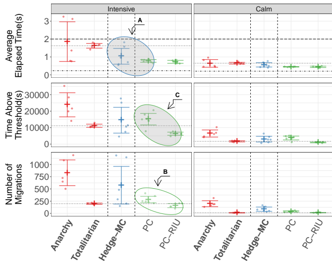
Fig. 17: Performance Evaluation for Greedy Strategies in the Affinity Scenario. The strategies in bold (Anarchy, Totalitarian and Hedge-MC) are kept as a basis for comparison. Note that the y-axis scale has changed.
