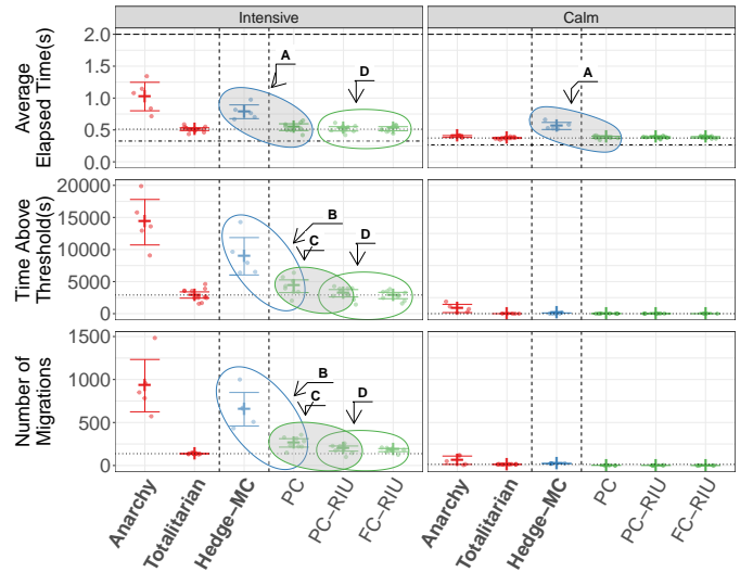
Fig. 15: Performance Evaluation for Greedy Strategies. The strategies in bold (Anarchy, Totalitarian and Hedge-MC) are kept as a basis for comparison. Note that the y-axis scale has changed.
