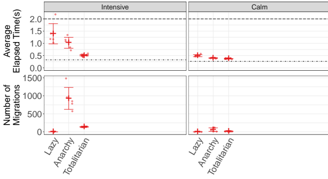
Fig. 9: Performance Evaluation for Baseline Strategies. The 2s horizontal dashed line represents the satisfaction threshold, while the bottom line represents the minimum response time when operating on a dedicated server.
