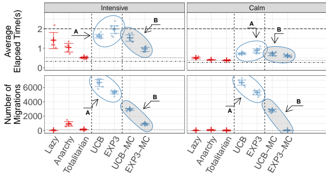
Fig. 10: Performance Evaluation for UCB, EXP3, UCB-MC and EXP3-MC Strategies. Note that the y-axis scale has changed and that a horizontal dotted line was added to indicate the performance of our target Totalitarian strategy.
