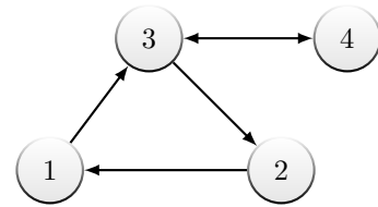
Fig. 1. Communication graph of the distributed observer.
