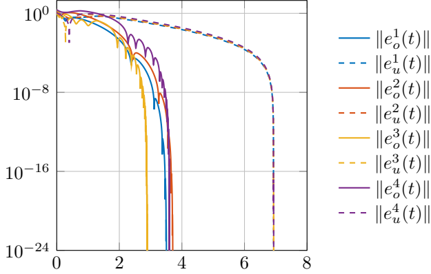
Fig. 2. Errors of the observer network in transformed coordinates.
