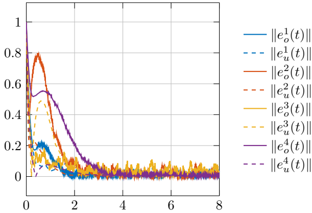
Fig. 3. Errors of the observer network in transformed coordinates in case of measurement noise.
