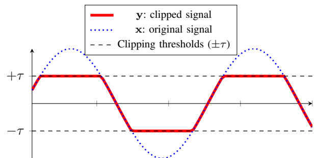
Figure 1. Hard-clipping model (1)
