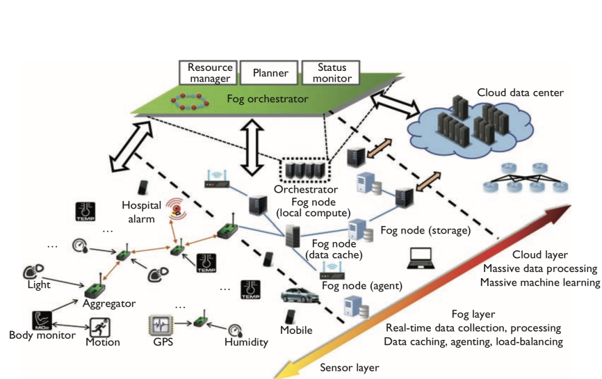
Figure 1: Generic Fog computing architecture [152].
