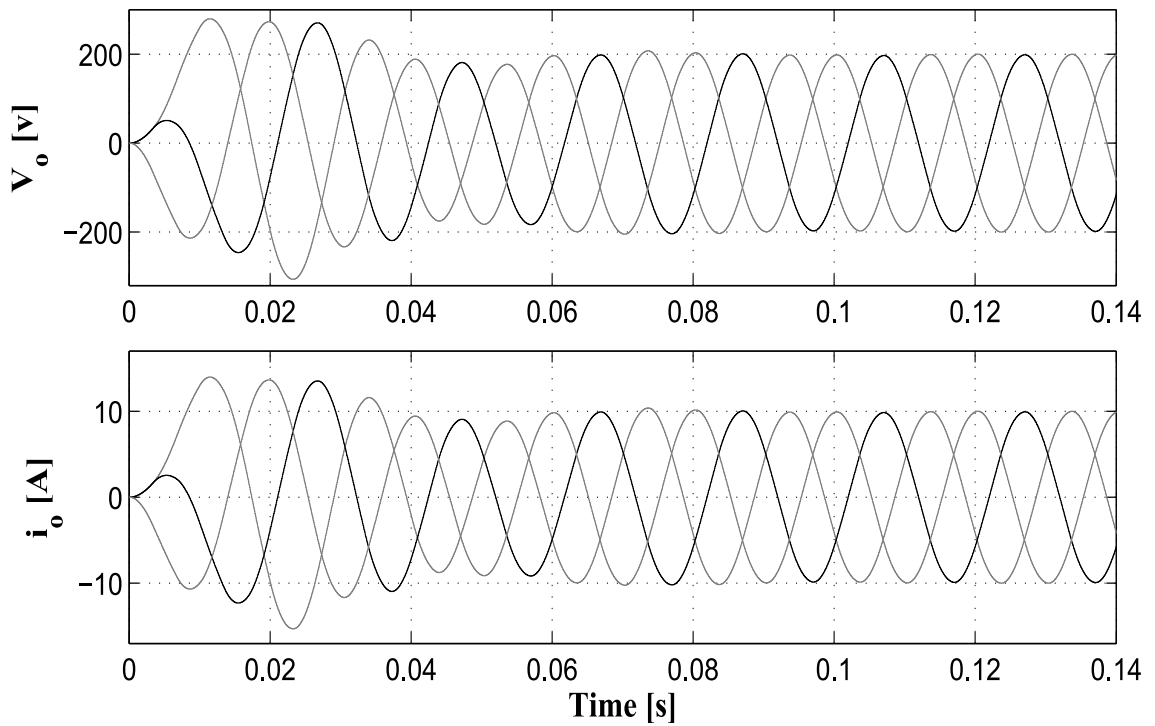
Figure 5.38: The experimental three phase output voltages and currents for a MPC with resistive load of 20\text{-}\Omega load. Voltage THD: 0.7%.
