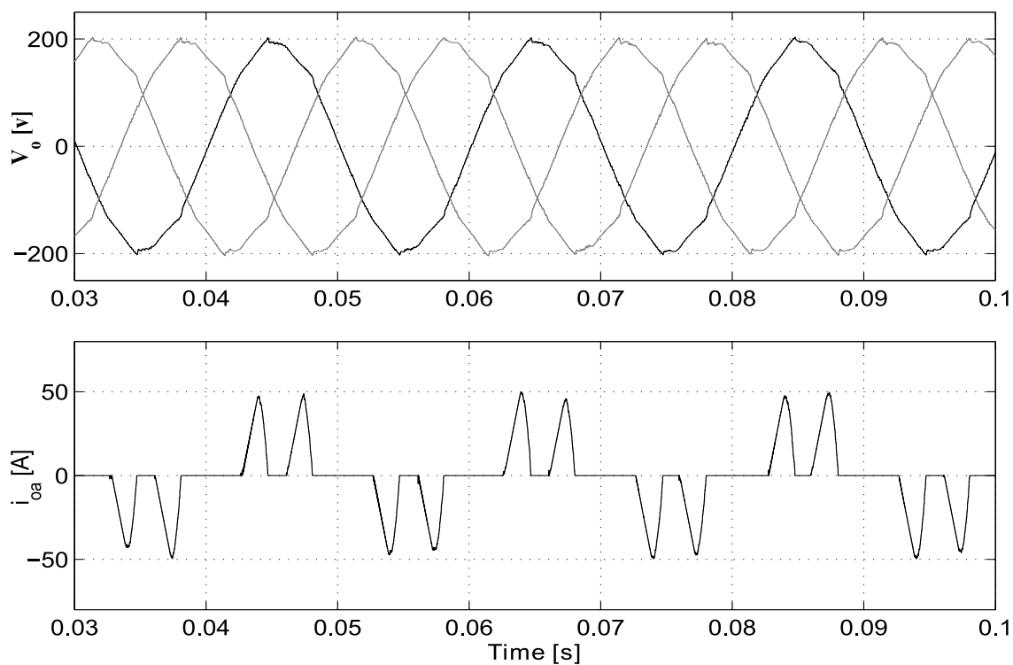
Figure 5.7: The simulated three phase output voltages and currents at steady state for a nonlinear load with a sampling time of T_s = 10 \mu s . Voltage THD: 2.18%.
