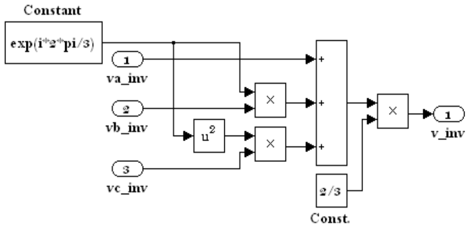
Figure 4.2: The simulation model of the voltage vector v_i .
