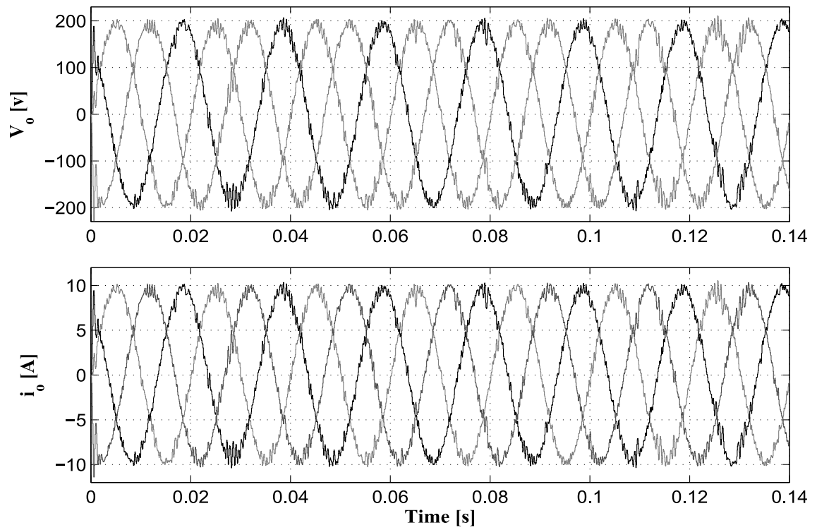
Figure 5.45: The simulated three phase output voltages and currents for a MPC with resistive load of 20\text{-}\Omega and according to the previous modifications. Voltage THD: 6%.
