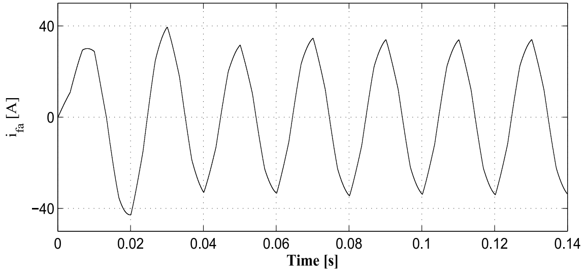
Figure 5.44: The experimental filter current for a MPC with a nonlinear load. Current THD: 3.07%.
