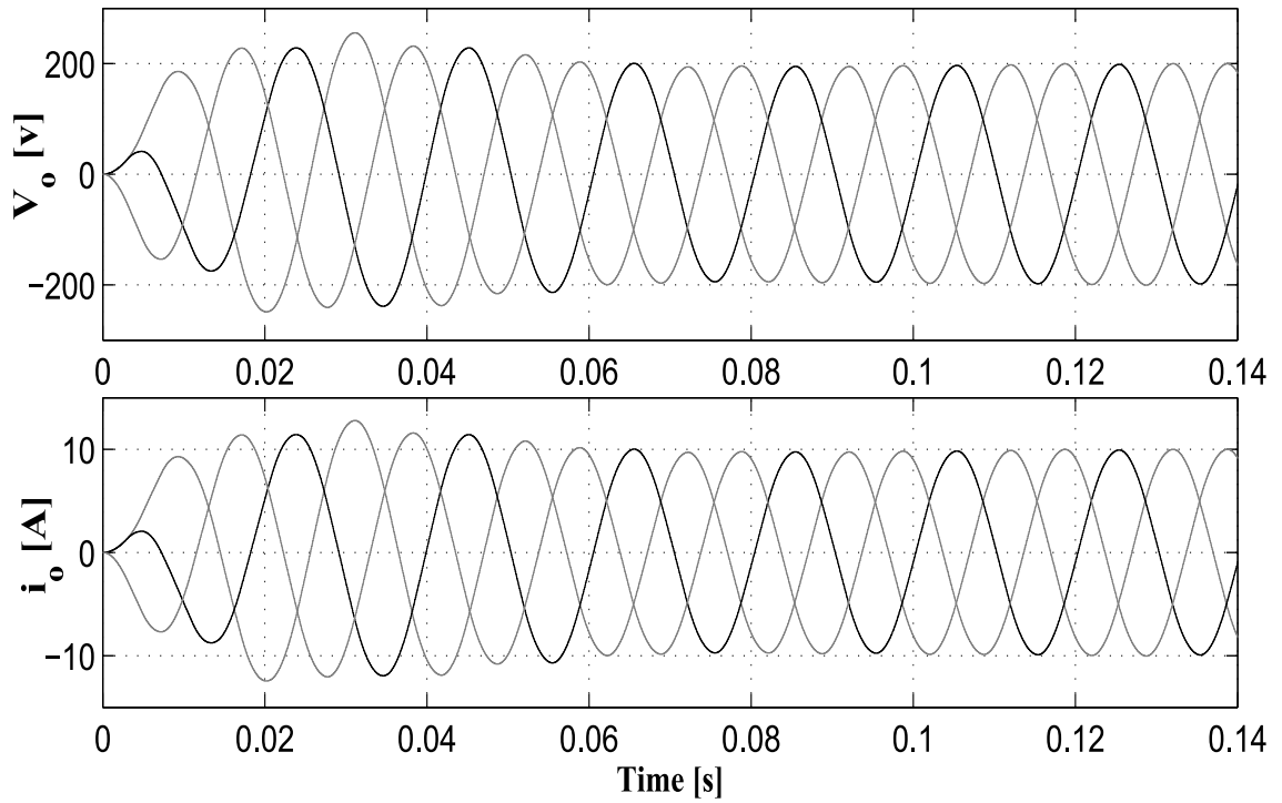
Figure 5.37: The simulated three phase output voltages and currents for a MPC with resistive load of 20\text{-}\Omega load. Voltage THD: 0.57%.
