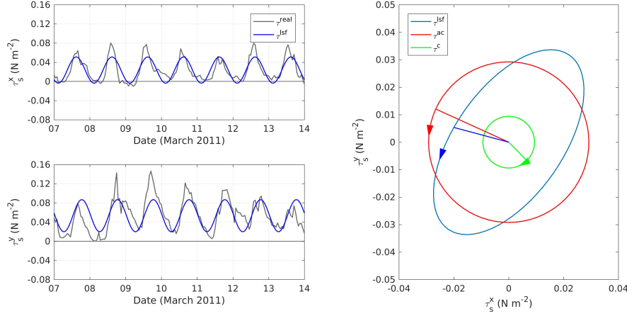
Figure 2. Rotary analysis of wind stress over an example
