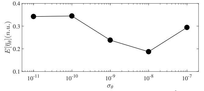
Fig. 2. Average of mean absolute parameter estimation error E[\bar{\eta}_\theta] in the ORD model as a function of the standard deviation of the process noise \sigma_\theta .
