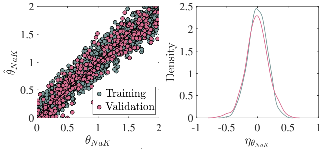
Fig. 1. Left panel: Estimated ( \hat{\theta}_{NaK} ) vs actual ( \theta_{NaK} ) values of the factor multiplying maximal I_{NaK} in the training and validation populations. Right panel: Density of the absolute error in the estimation of \theta_{NaK} for the training and validation sets.
