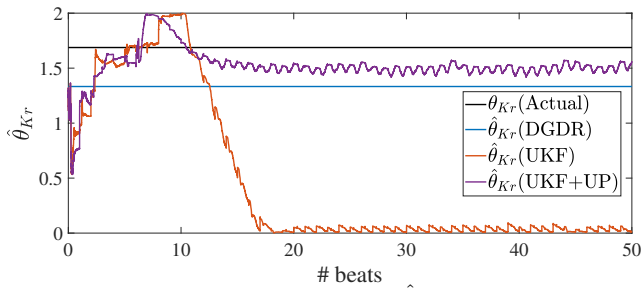
Fig. 4. Actual \theta_{Kr} value and time course of \hat{\theta}_{Kr} as estimated by DGDR, UKF and UKF+UP methods.
