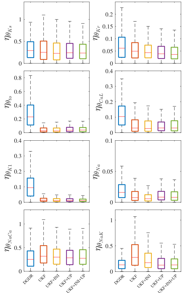
Fig. 6. Boxplots of absolute estimation errors \eta_\theta for the factors multiplying ionic current conductances calculated for the five evaluated methods.
