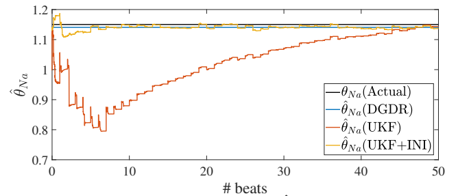
Fig. 3. Actual \theta_{Na} value and time course of \hat{\theta}_{Na} as estimated by DGDR, UKF and UKF+INI methods.
