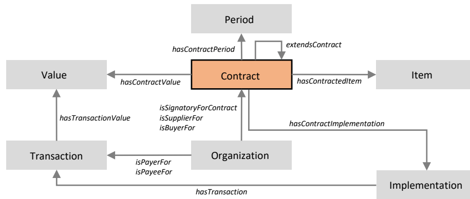
Fig. 5. Contract class and its neighbourhood.
