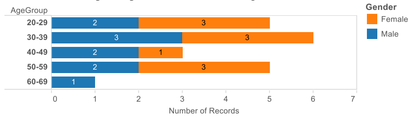
Fig. 1. Age Distribution
