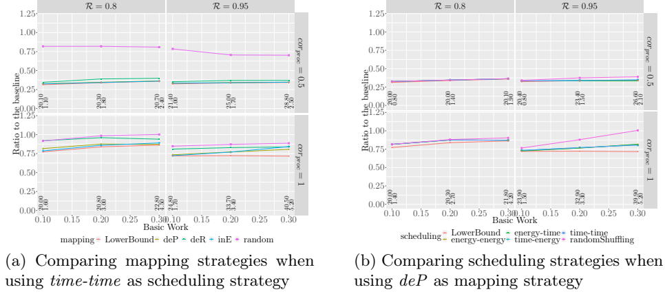
Figure 6: Ratio of energy consumption using different mapping and scheduling strategies when varying basicWork and \mathcal{R}_i , under big failure rate, with \beta_{b/w} = 1 and cor_{task} = 0.5 .
