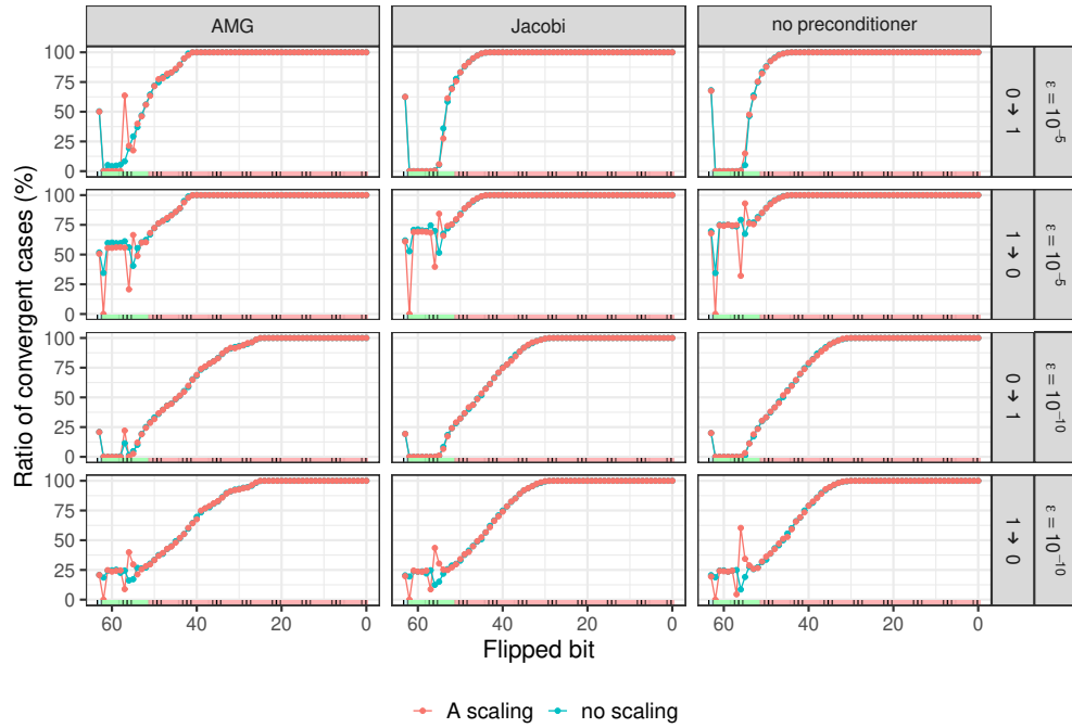
Figure 1.1: Comparison of the impact on convergence of the bit-flips at originally zero or one bits. The 64-bit indices of the IEEE 754 floating point numbers are displayed between each graph; from left to right, the sign (blue), exponent (green) and mantissa (red) bits are represented.
