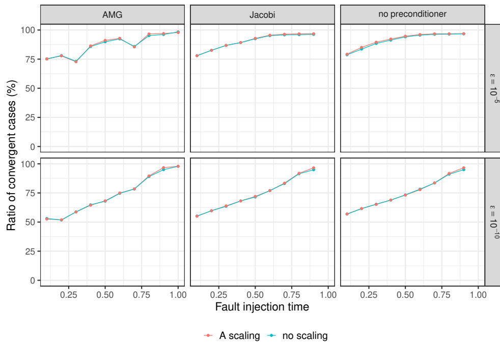
Figure 1.3: Impact of the bit-flip injection time (as a proportion of the number of iterations with respect to the non-faulty execution) in the matrix-vector product on PCG convergence success.
