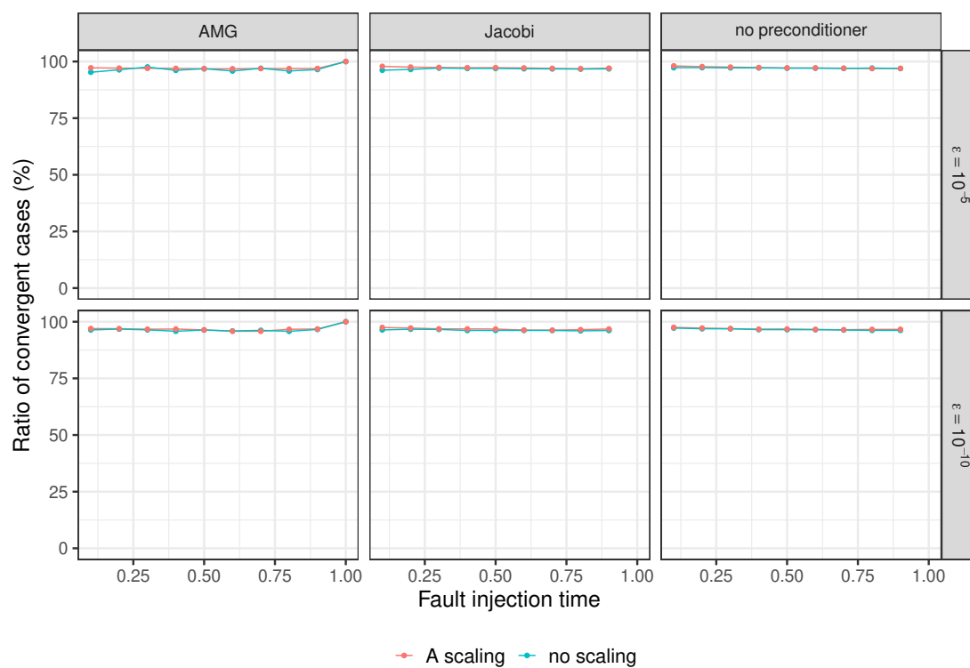
Figure 3.7: Impact of the bit-flip injection time in the preconditioner application on PCG convergence success. Recall that no preconditioner means M = I .
