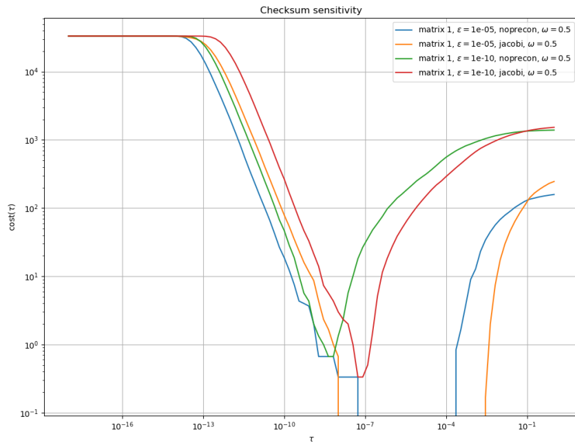
Figure 2.2: Cost function for a given matrix, and \omega , but with different combinations of \epsilon and preconditioner.
