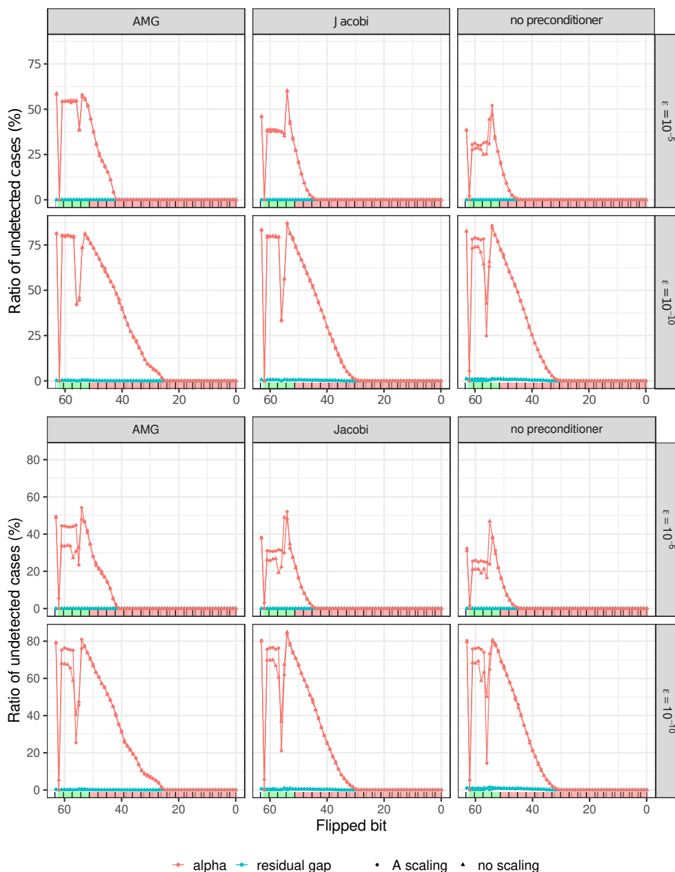
Figure 5.1: Detection performance of the residual gap and \alpha -based methodologies for soft errors in the matrix-vector product calculation. (top) Early bit-flips (in r_{i+1} ). (bottom) Late bit-flips (in u_{i+1} ).
