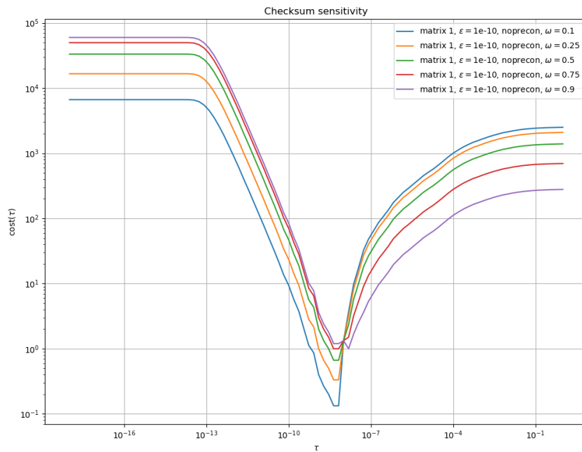
Figure 2.1: Cost function for a given matrix, \varepsilon , and preconditioner, but with different values of \omega .
