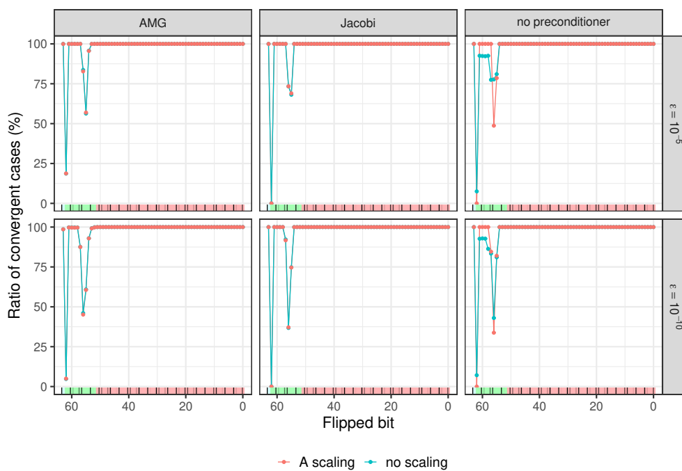
Figure 1.4: Impact of the index of the flipped bit in the preconditioner application on PCG convergence success.
