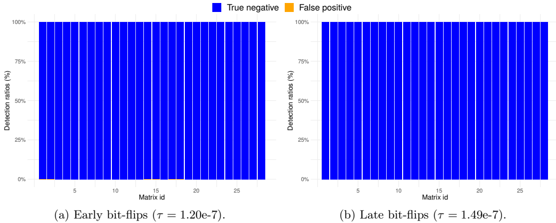
Figure 3.2: Outcome of the checksum-based detection for the non-faulty runs when using the non-optimal thresholds \tau for early (in p_i ) and late (in s_i ) bit-flips, considering only the experiments with a Jacobi preconditioner and \varepsilon = 1e-10 ( \omega = 0.5 ).
