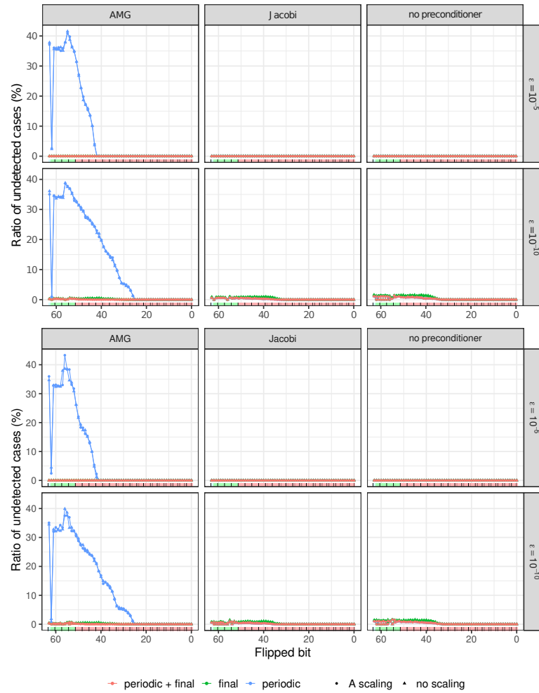
Figure 4.1: Detection performance of the three policies based on the residual gap criterion. (top) Early bit-flips (in p_i ). (bottom) Late bit-flips (in s_i ).
