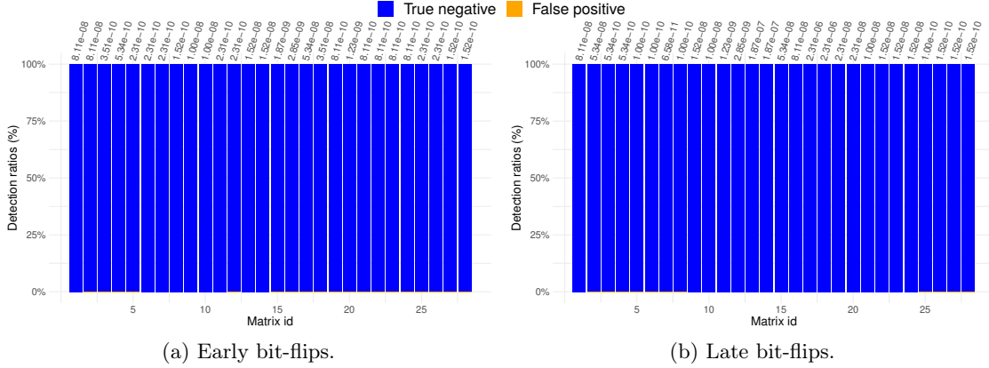
Figure 3.1: Outcome of the checksum-based detection for the non-faulty runs when using the optimal thresholds \tau (top of the bars) for early (in p_i ) and late (in s_i ) bit-flips, considering only the experiments with a Jacobi preconditioner and \varepsilon = 1e-10 ( \omega = 0.5 ).
