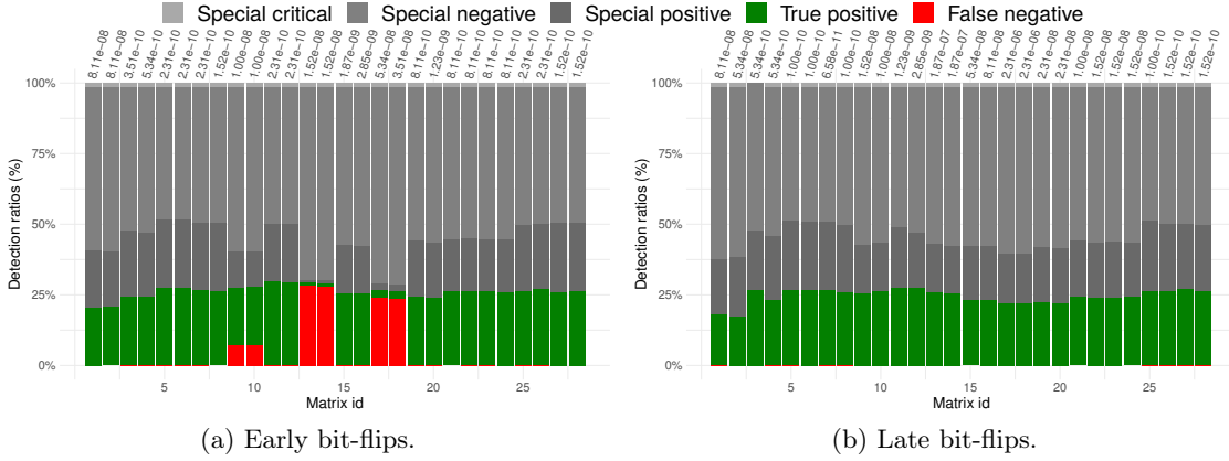
Figure 4.1: Outcome of the checksum-based detection for the faulty runs when using the optimal thresholds \tau (top of the bars) for early (in p_i ) and late (in s_i ) bit-flips, considering only the experiments with a Jacobi preconditioner and \varepsilon = 1e-10 ( \omega = 0.5 ).
