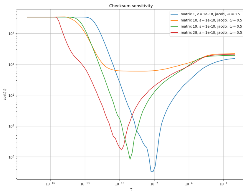
Figure 2.3: Cost function for a given \varepsilon , preconditioner, and \omega , but for different matrices.
