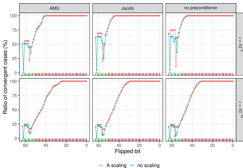
Figure 1.2: Impact of the index of the flipped bit in the matrix-vector product on PCG convergence success. The 64-bit indices of the IEEE 754 floating point numbers are displayed between each graph; from left to right, the sign (blue), exponent (green) and mantissa (red) bits are represented.
