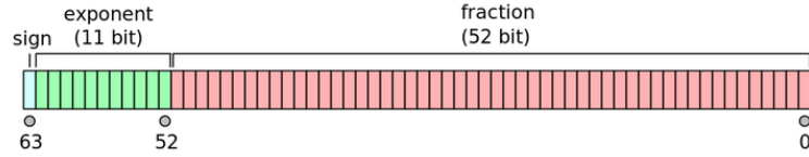
Figure 2.1: IEEE 754 double-precision binary floating-point format.
