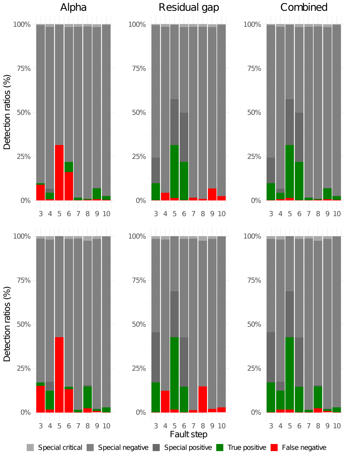
Figure 4.5: Comparison of the detection success of the alpha and residual gap based methodologies, and their combination for bit-flips in all possible steps of PCG. The set PCG runs used for this experiment is different from the other experiments, but was created using the same methodology described in Section 3.2. The only difference is the possible locations for the bit-flip. (top) Early bit-flips. (bottom) Late bit-flips.
