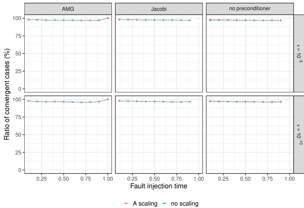
Figure 1.5: Impact of the bit-flip injection time in the preconditioner application on PCG convergence success.
