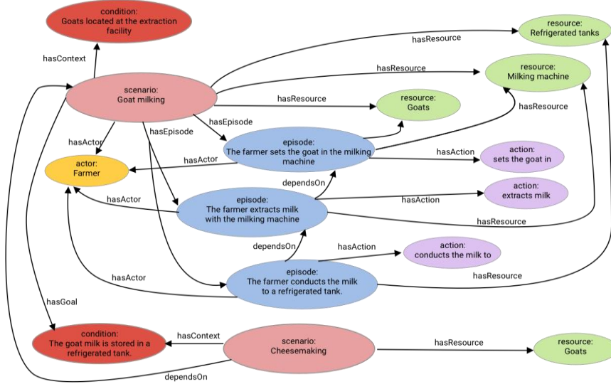
Figure 1. Classes and dependencies
