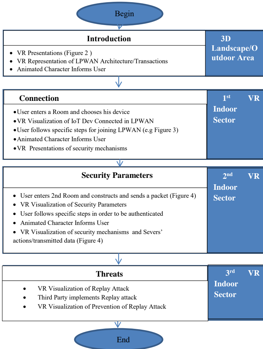
Fig. 1. VR Training Phases.
