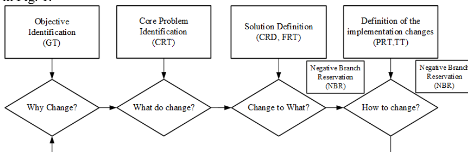
Fig. 1. The TOC Basic Questions and TOC TP tools
