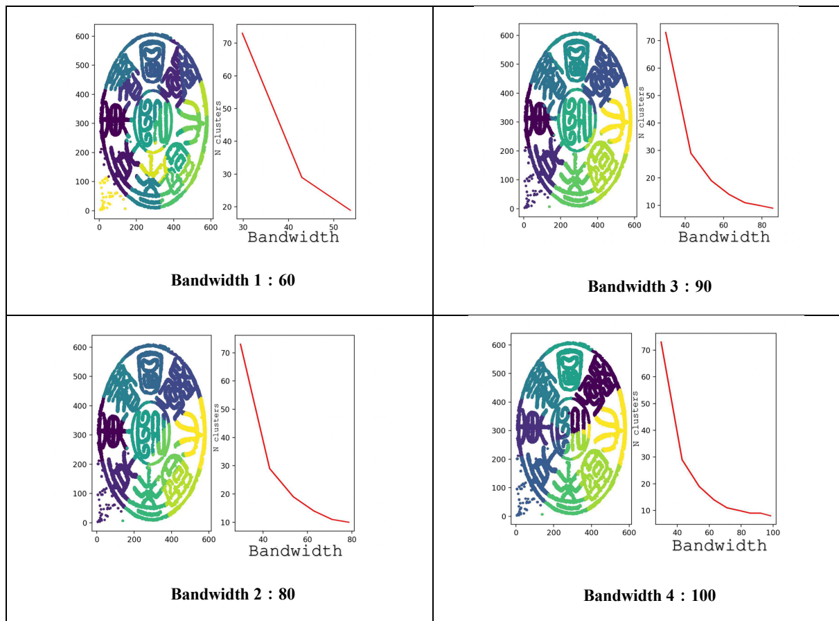
Figure 7. Visualization of clustering results under different bandwidths.
