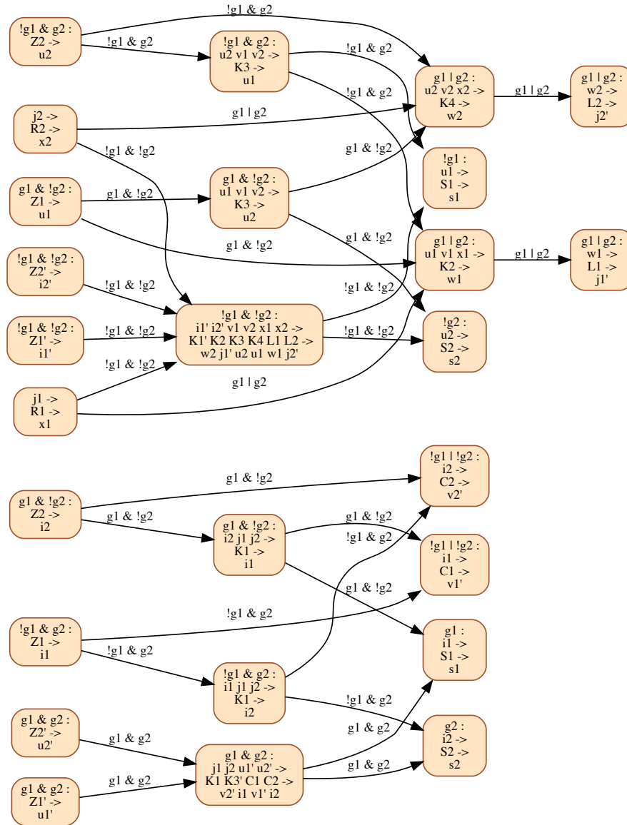
Figure 11: Block dependency graph of the RLDC2 model, generated by IsamDAE. Vertices are labeled p : R \rightarrow B \rightarrow W , where: p is a propositional formula defining in which modes the block is evaluated; R is the set of variables to read; B is the set of equations of the block; W is the set of variables to write. Edges are labeled by a propositional formula, defining in which modes the dependency applies.
