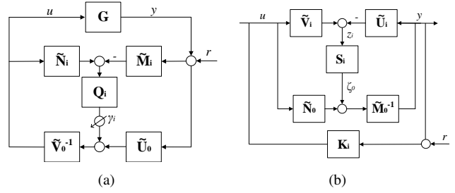
Fig. 2. (a) YK parameterization for controller reconfiguration and (b) Dual YK parameterization for CL identification.
