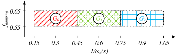
Fig. 5. Uncertainty range string stable for pairs (\mathbf{G}_0, \mathbf{K}_0) , (\mathbf{G}_1, \mathbf{K}_1) and (\mathbf{G}_2, \mathbf{K}_2) .
