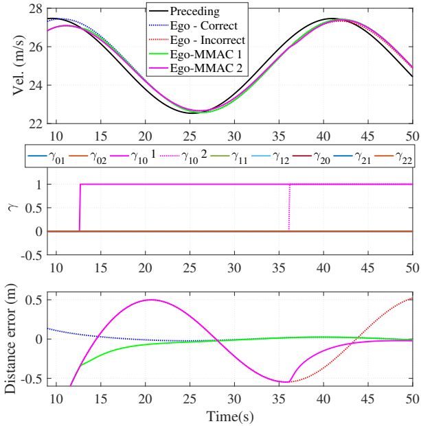
Fig. 9. Simulation results MMAC CACC. \mathbf{G}_{j-1} = \mathbf{G}_1 and \mathbf{G}_j = \mathbf{G}_{x3} .
