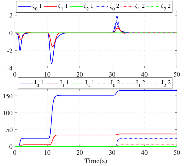
Fig. 6. \zeta_i and J_i comparison. \mathbf{G}_{j-1} = \mathbf{G}_0 and \mathbf{G}_j = \mathbf{G}_2 . Solid-line indicates the case where the system is activated at 0s, while dotted line shows the case where the system is activated at 29s.
