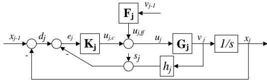
Fig. 3. CACC SISO structure.
