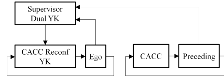
Fig. 1. Outline MMAC for CACC applications.
