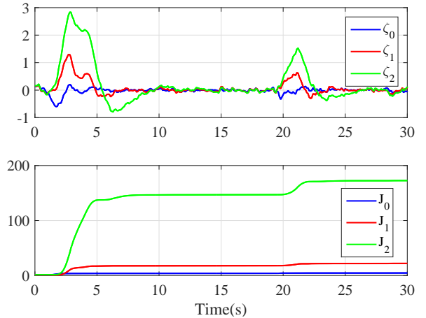
Fig. 12. \zeta_i and J_i comparison. Experimental results. Homogeneous string of two cycabs.
