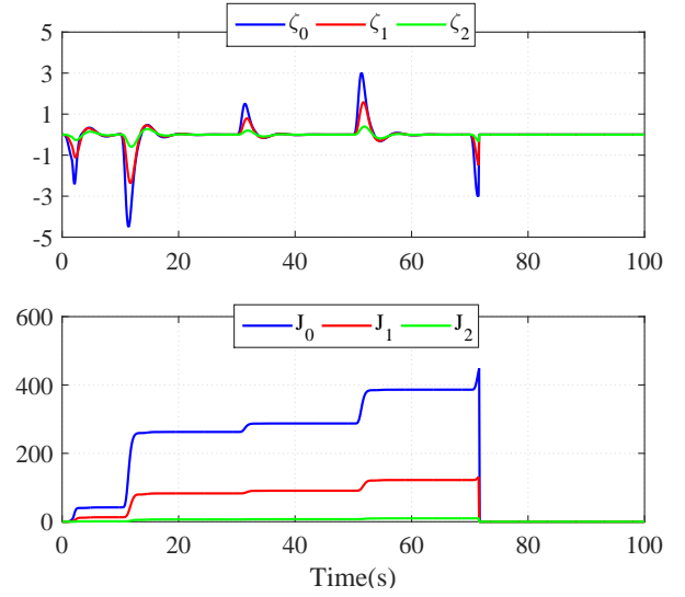
Fig. 10. \zeta_i and J_i comparison. \mathbf{G}_{j-1} = \mathbf{G}_{x1} and \mathbf{G}_j = \mathbf{G}_{x2} . System shutdown at 71.5s.
