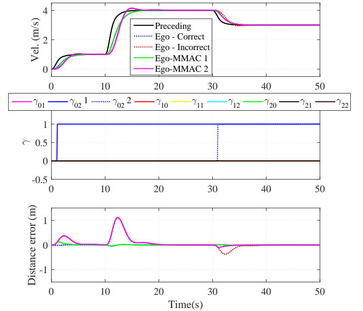
Fig. 7. Simulation results MMAC CACC. \mathbf{G}_{j-1} = \mathbf{G}_0 and \mathbf{G}_j = \mathbf{G}_2 .
