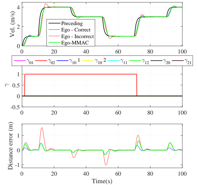
Fig. 11. Simulation results MMAC CACC. \mathbf{G}_{j-1} = \mathbf{G}_{x1} and \mathbf{G}_j = \mathbf{G}_{x2} . System shutdown at 71.5s.
