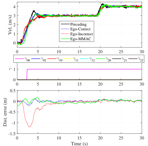
Fig. 13. Experimental results MMAC CACC. Homogeneous string of two cycabs.
