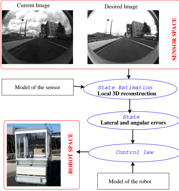
Fig. 3: Route following process with a visual sensor.
