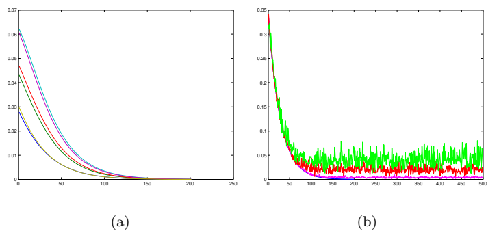
Figure 4: Control using joint sensors: (a) Joint velocities. (b) Robustness to noise : sum of squares of the errors E^T E with a noise amplitude of 0 deg, 0.01 deg, 0.05 deg and 0.1 deg.
