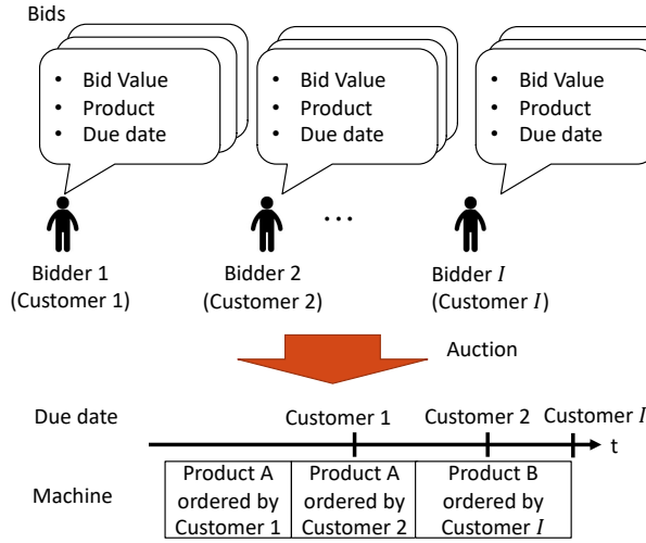
Fig. 1. Schema of Scheduling Auction
