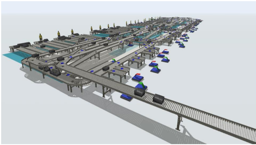
Fig. 2. The full-scale computer simulation model for the installed modular conveyor system.
