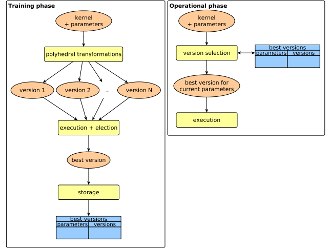
Figure 1. Overview of the multi-versioning training and operational phases
