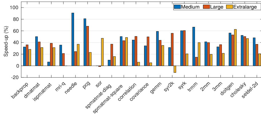
Figure 5. Speed-up with 100 invocations against Apollo without multi-versioning (Magerit: 20 threads/cores)
