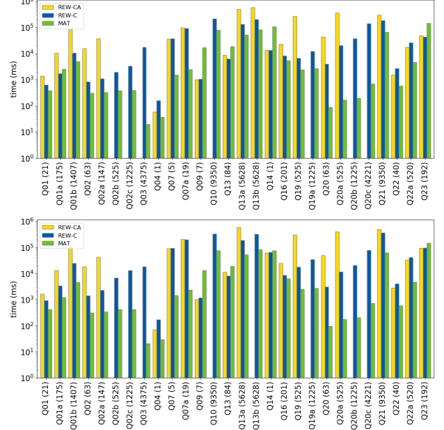
Figure 6: Query answering times on the larger RIS S_2 (top, relational sources) and S_4 (bottom, heterogeneous sources).
