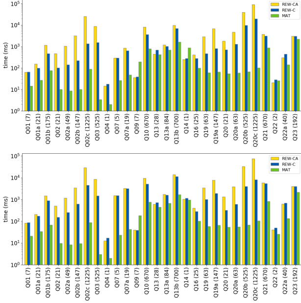
Figure 5: Query answering times on the smaller RIS S_1 (top, relational sources) and S_3 (bottom, heterogeneous sources).
