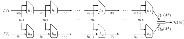
Fig. 2: The concatenation combiner
