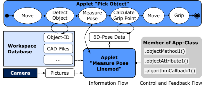
Fig. 2. Exemplary interaction of strategic applets within a skill-based system
