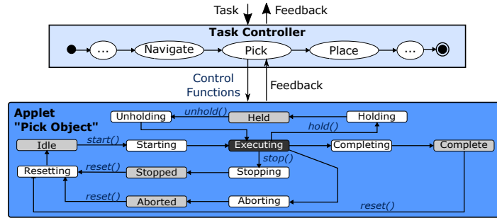
Fig. 3. Task controller interacting with an applet
